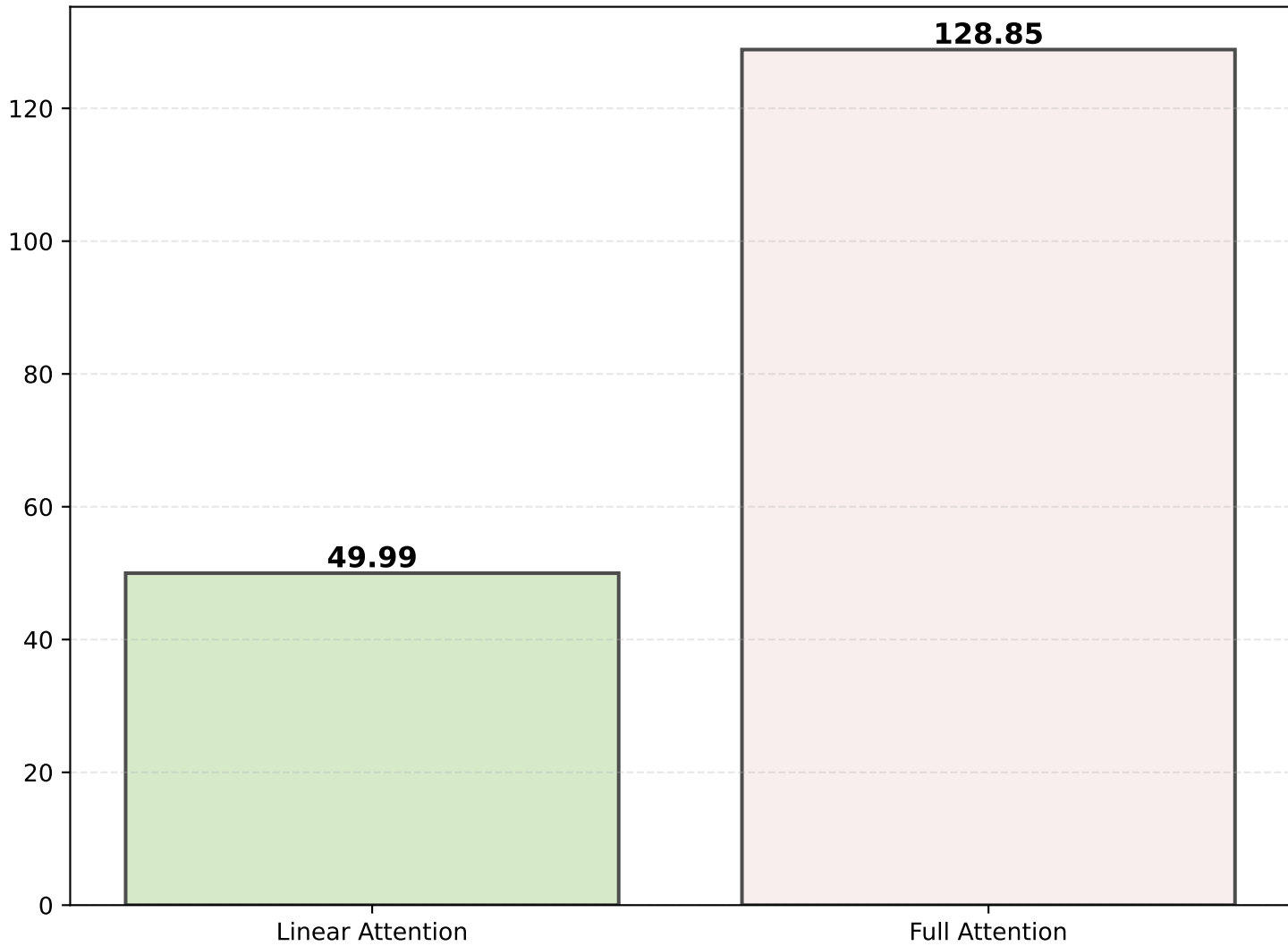
FLOPs Comparison
