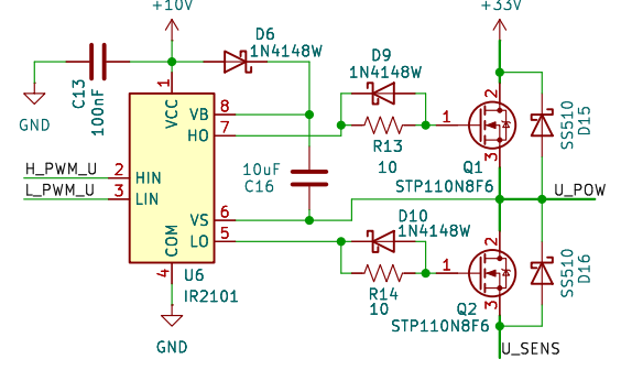
MOSSFET and drivers(6PWM)
