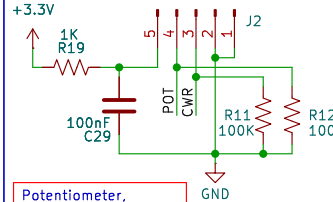
Torque control connector
