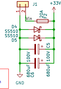
Motor connector
