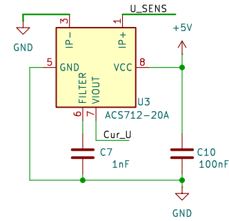
Current sensors(isolated)
