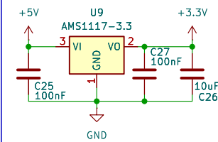
3.3V linear power supply
