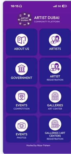
Figure 6.1: Current layout with "About Us" in top-left position versus recommended task-oriented hierarchy.
