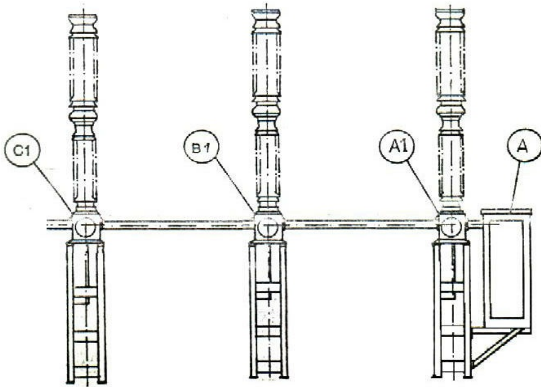
Figure 1 : HPL 123-170/25.1-40.1 and HPL 245-300/25B1-31B1 Three Pole operated Circuit Breaker mounted on a three-column Framework
