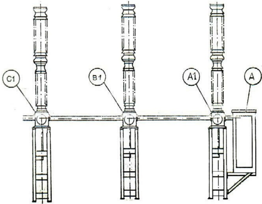
Figure 1 : HPL 123-170/25.1-40.1 and HPL 245-300/25B1-31B1 Three Pole operated Circuit Breaker mounted on a three-column Framework
