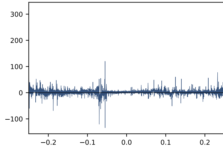
C_3 construction ( n = 100000 , OrganonAgent)
