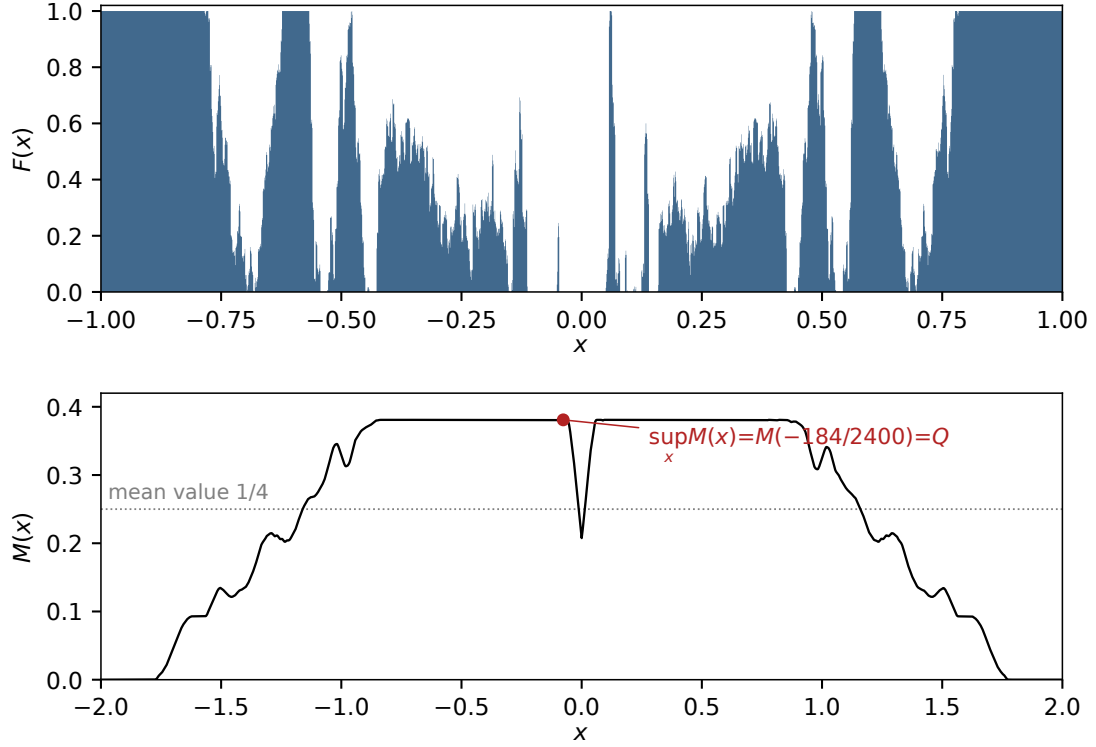
Figure 1: The certified construction. Top : the exactly rescaled Hyra step function F on [-1, 1] ( n = 2400 cells). Bottom : its overlap function M on [-2, 2] , continuous and piecewise linear with breakpoints on the lattice h\mathbb{Z} (Lemma 1), plotted through the 4801 lattice values M(mh) ; the dotted line is the mean value \frac{1}{4} of M on [-2, 2] . The maximum is attained at x^* = -184/2400 , where M(x^*) = Q . Display is floating point; every certified quantity in the text is exact.
