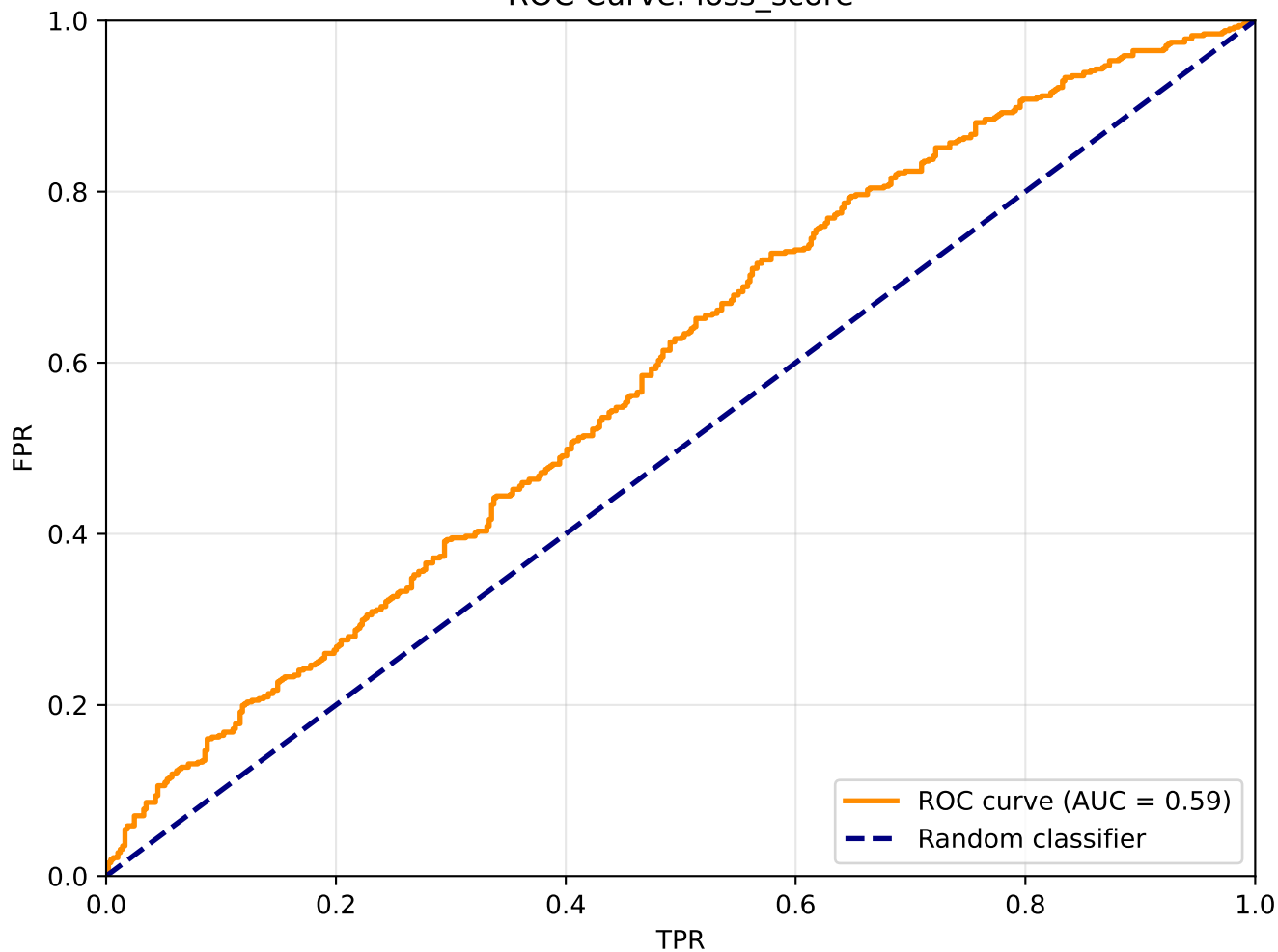
ROC Curve: loss_score
