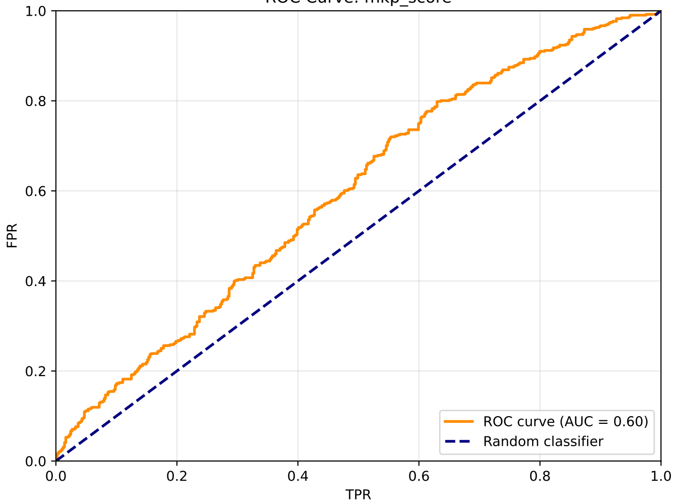
ROC Curve: mkp_score
