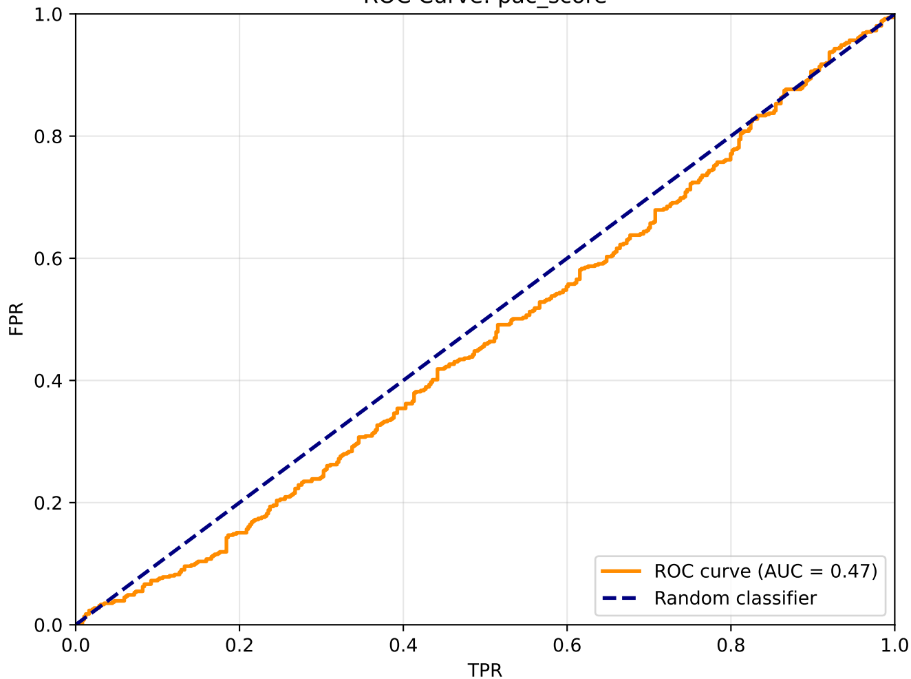
ROC Curve: pac_score
