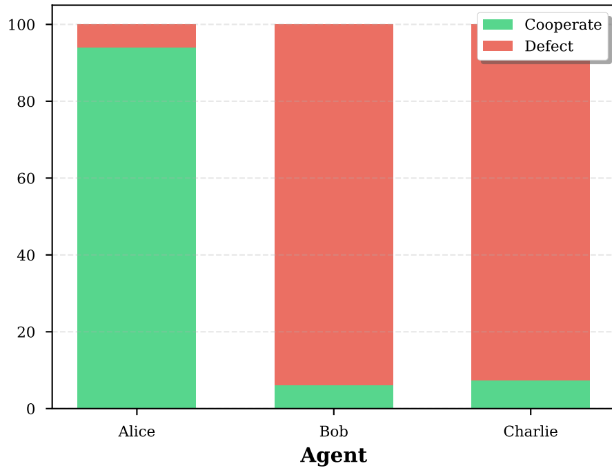
IPD - Agent Behavior
