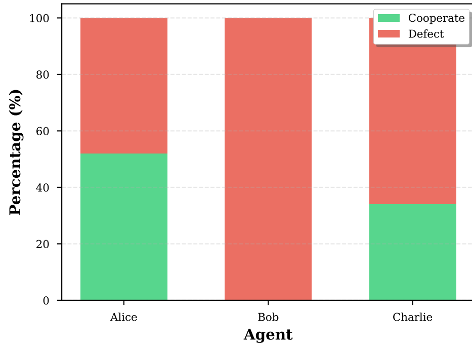
PGG - Agent Behavior
