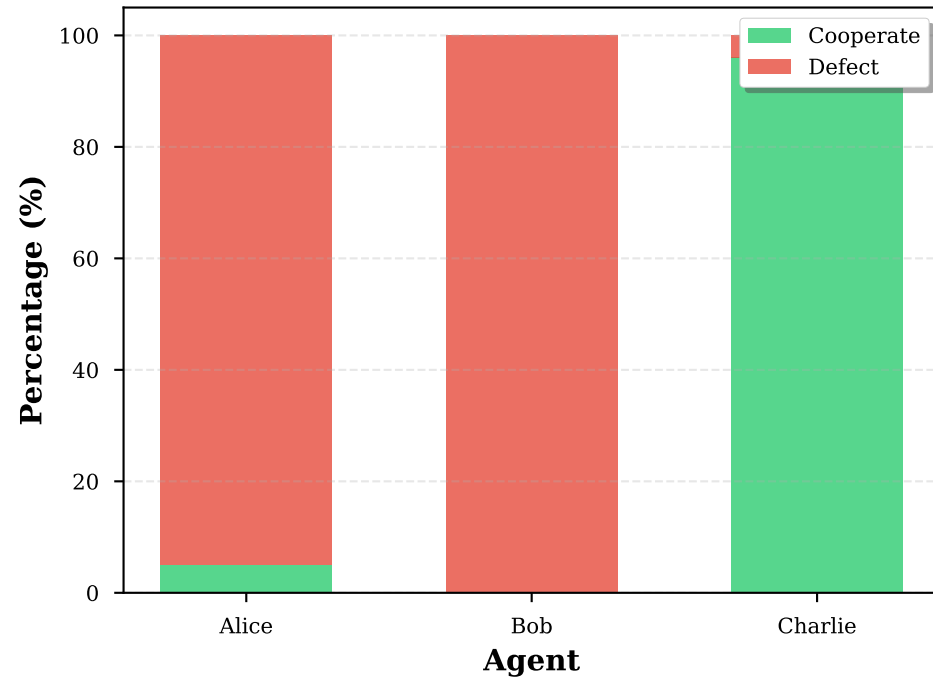
VD - Agent Behavior
