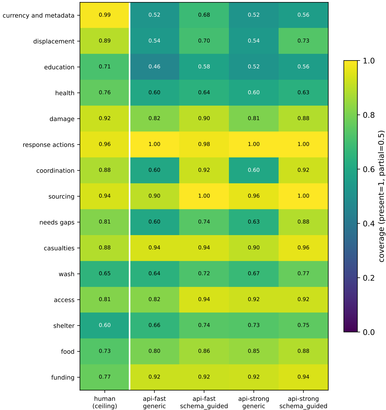
Slot coverage: human ceiling vs machine arms (rows ordered by human-machine gap)
