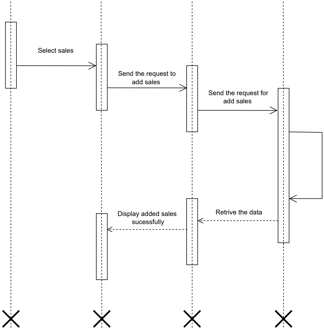
Sales interface
