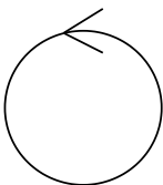
Client class
