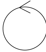
Reviews class
