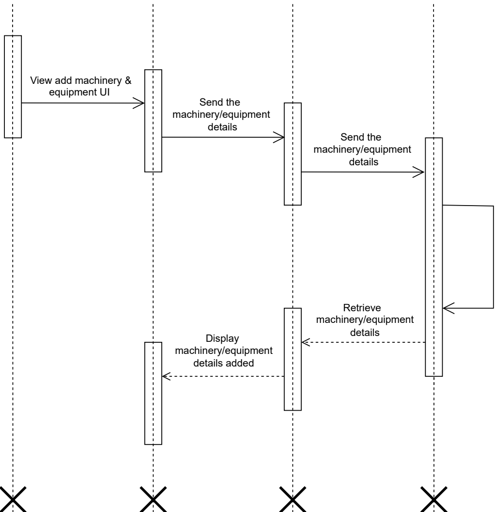
Add Machinery & Equipment UI
