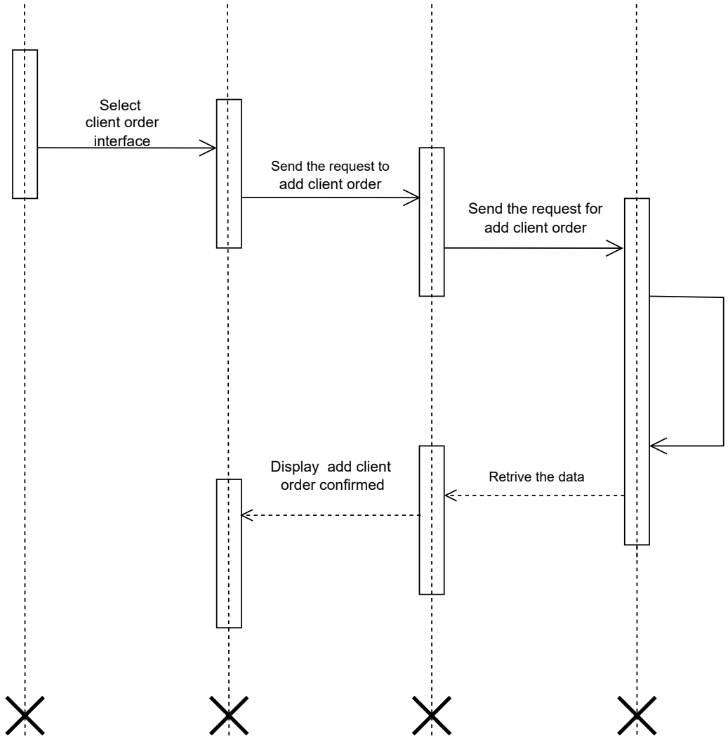
Client order interface
