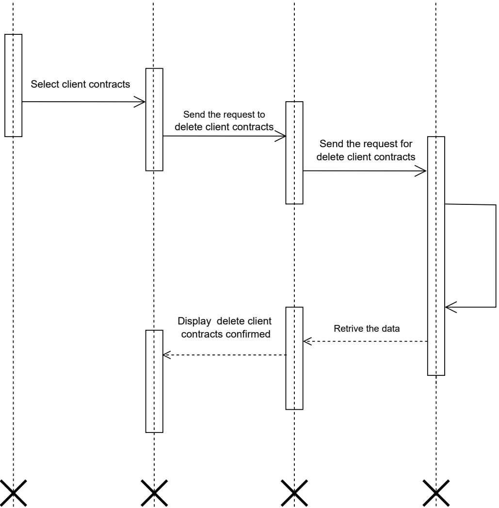
Delete client contracts interface
