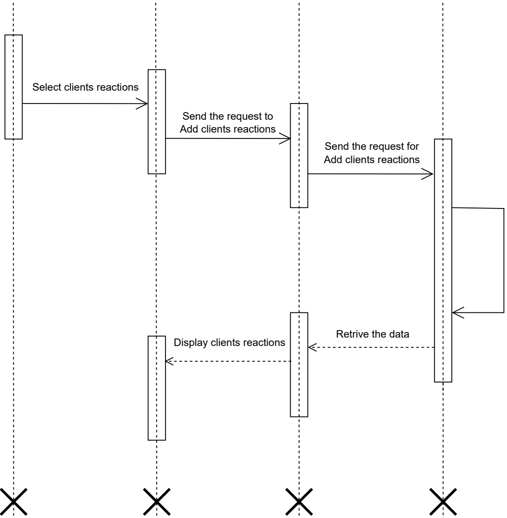
Clients reactions interface
