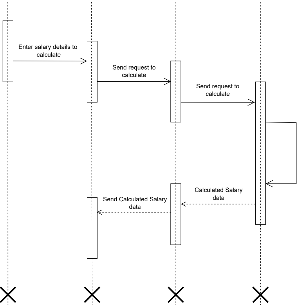
Calculate Salary UI
