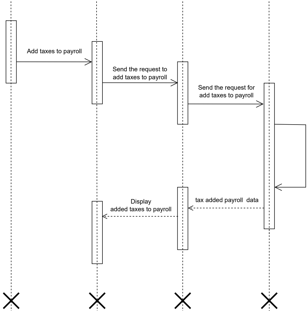
Add taxes to payroll UI
