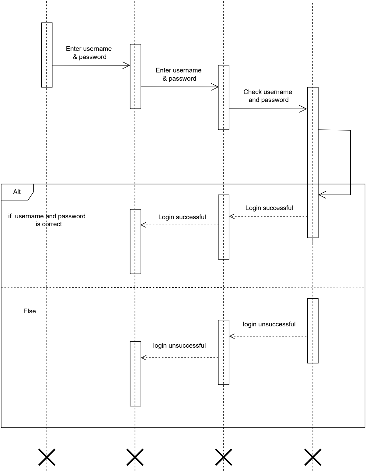
Client
