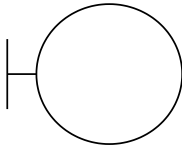
Cart interface
