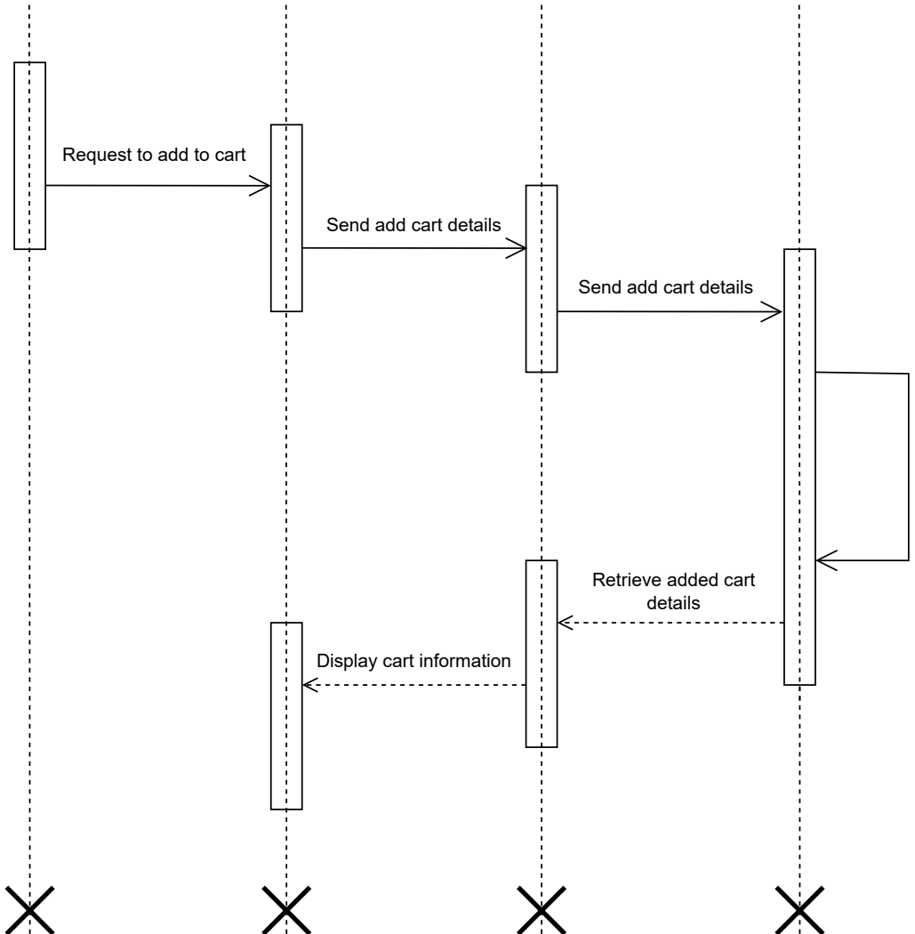
Cart interface
