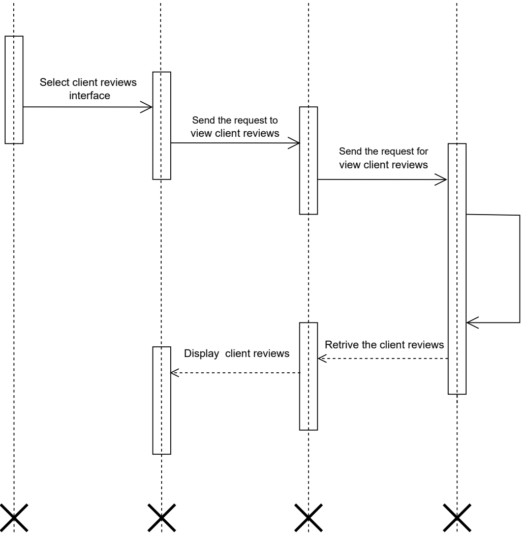
Reviews interface
