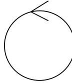
Sales class
