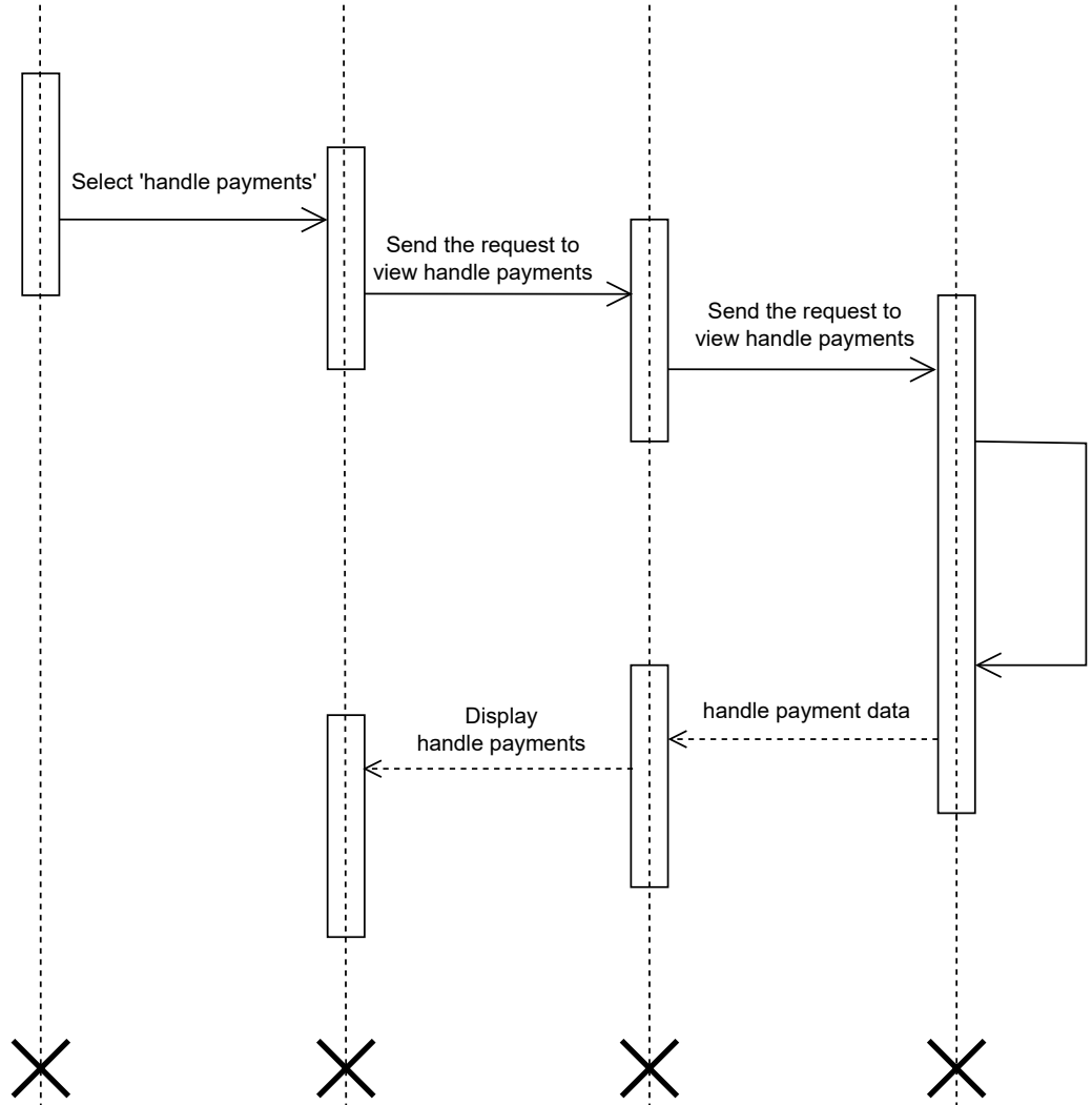
Handle payments UI
