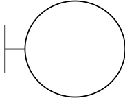
Cart interface
