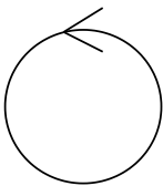
Feedback class
