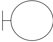
Sales interface
