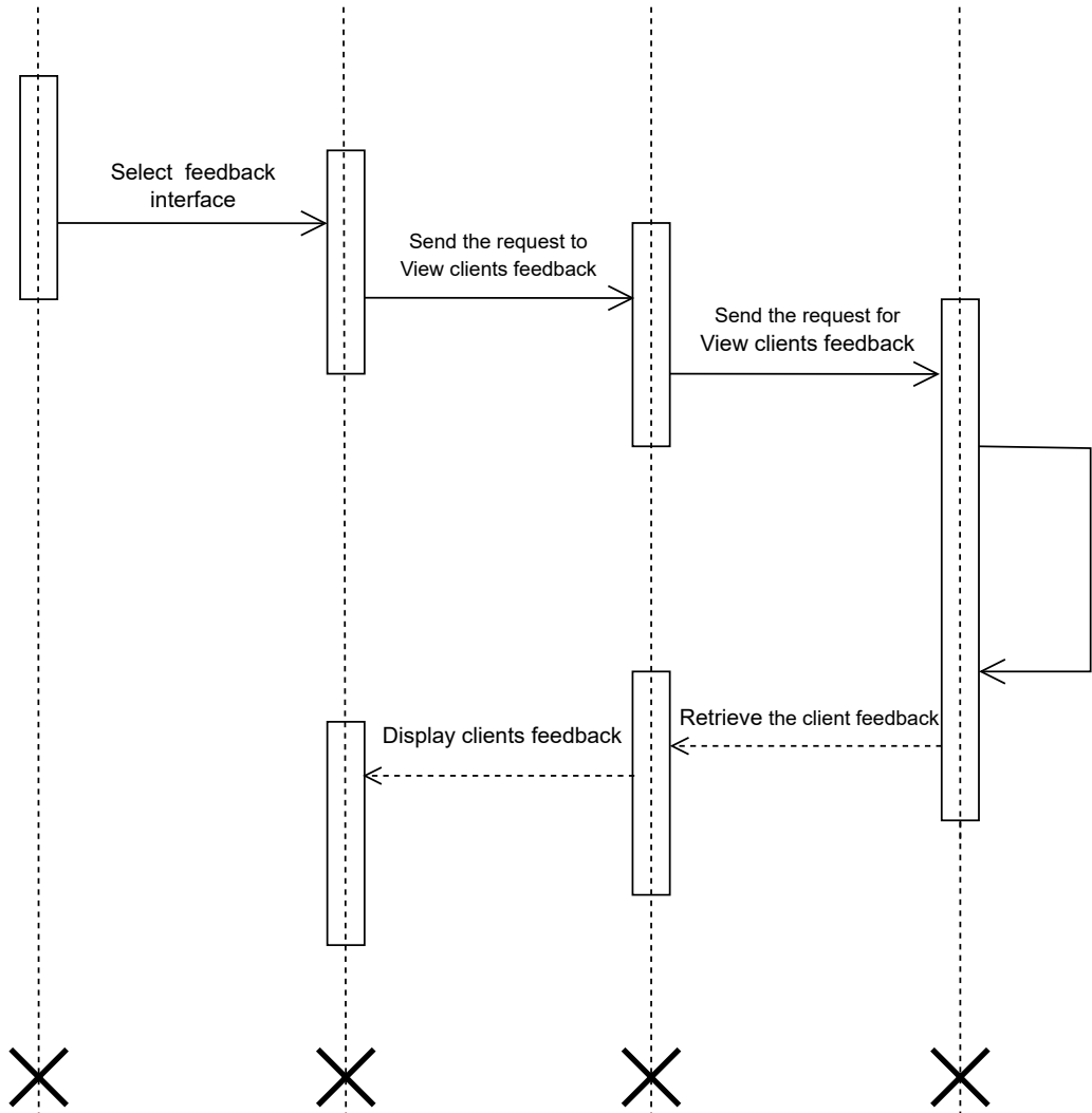
Feedback interface
