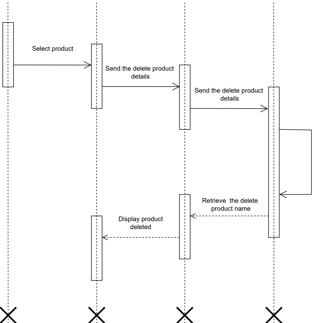
Delete Product interface
