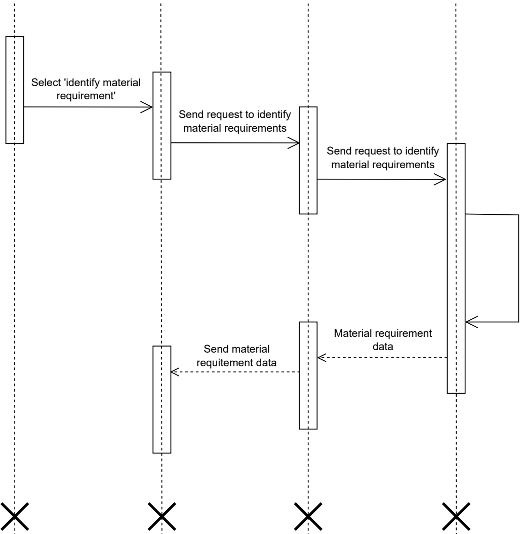
Identify material requirements UI
