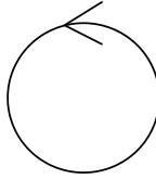
Cart Class
