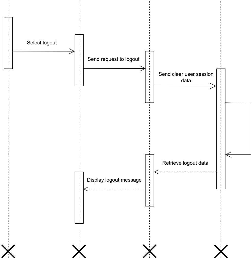
Logout interface
