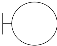
Feedback interface
