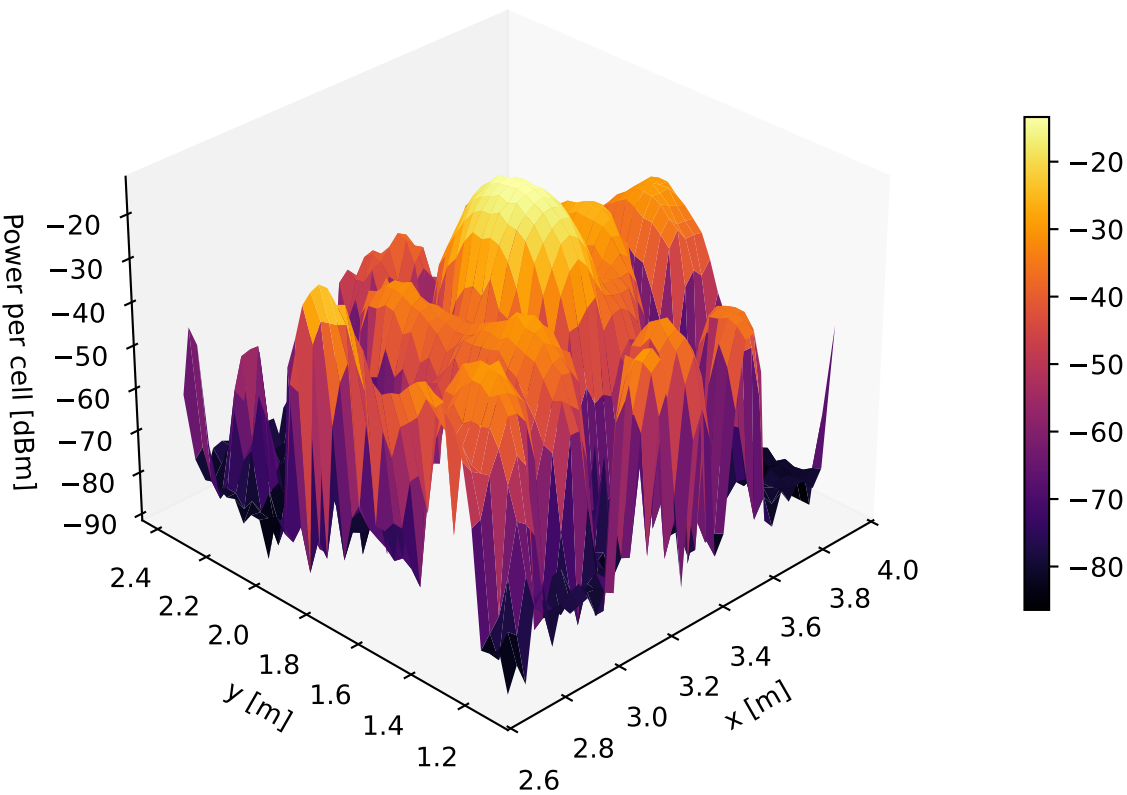
FRIIS-0 | mean power per cell [dBm] (3D)
