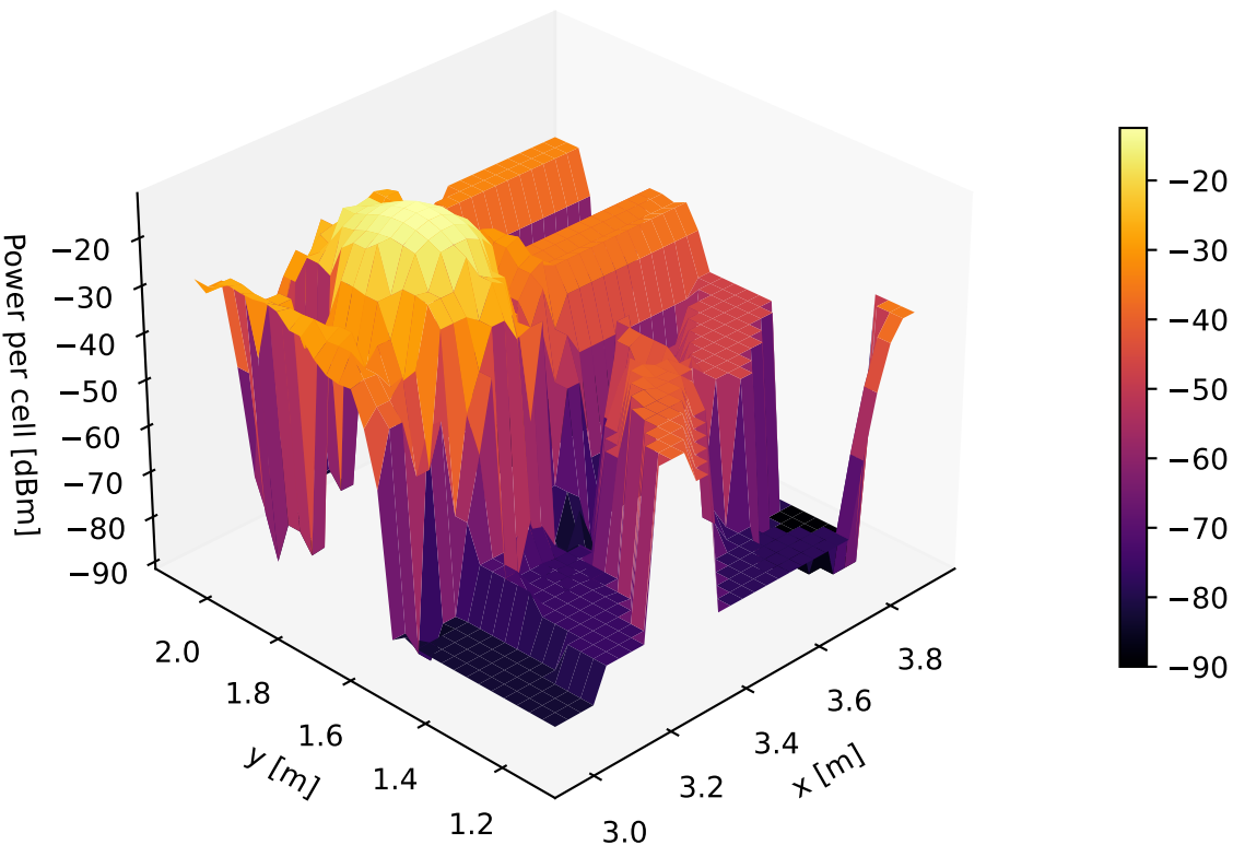
RECI-3 | mean power per cell [dBm] (3D)
