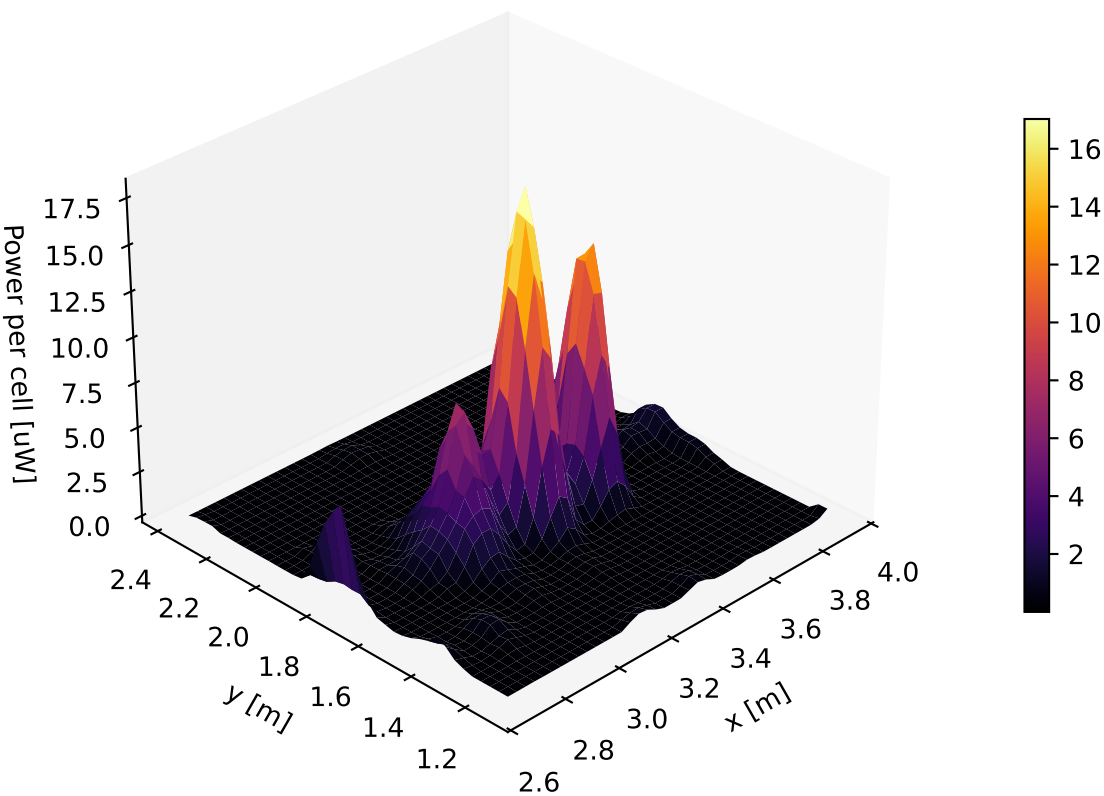
FRIIS-ABS-REFL-0 | mean power per cell [uW] (3D)
