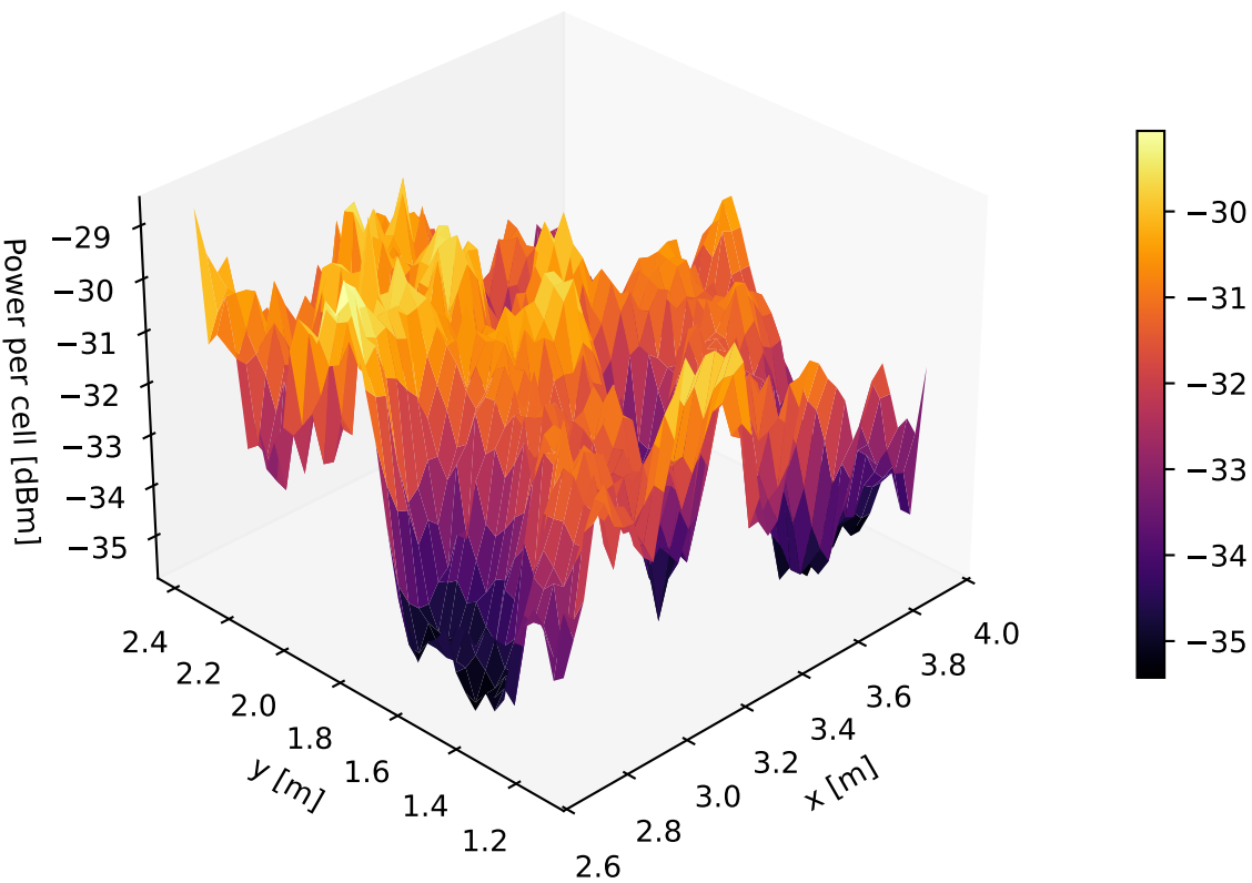
RANDOM-1 | mean power per cell [dBm] (3D)
