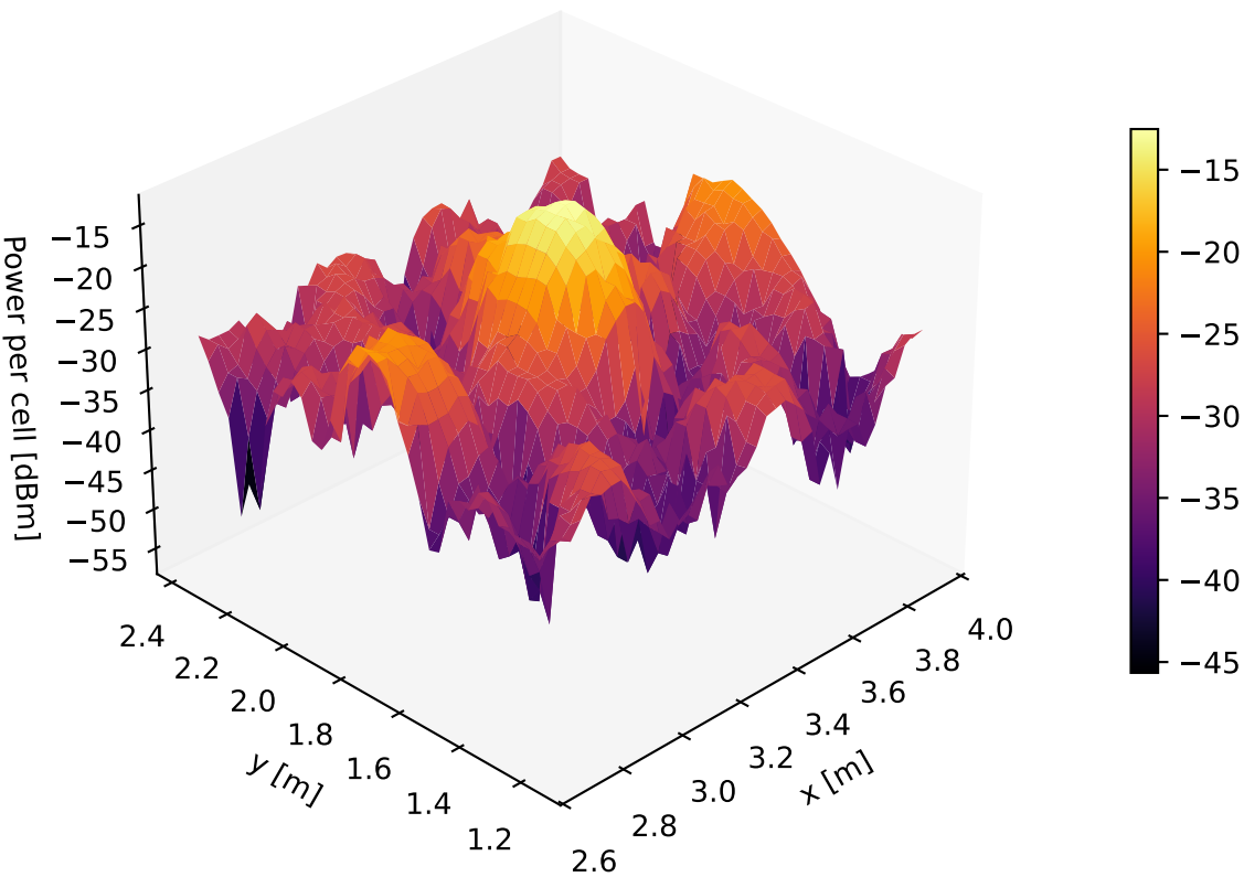
RECI-RF-1 | mean power per cell [dBm] (3D)
