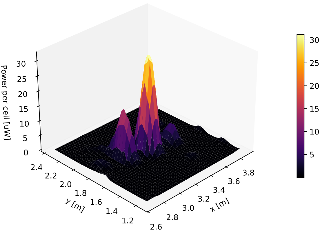
RECI-ABS-REFL-0 | mean power per cell [uW] (3D)
