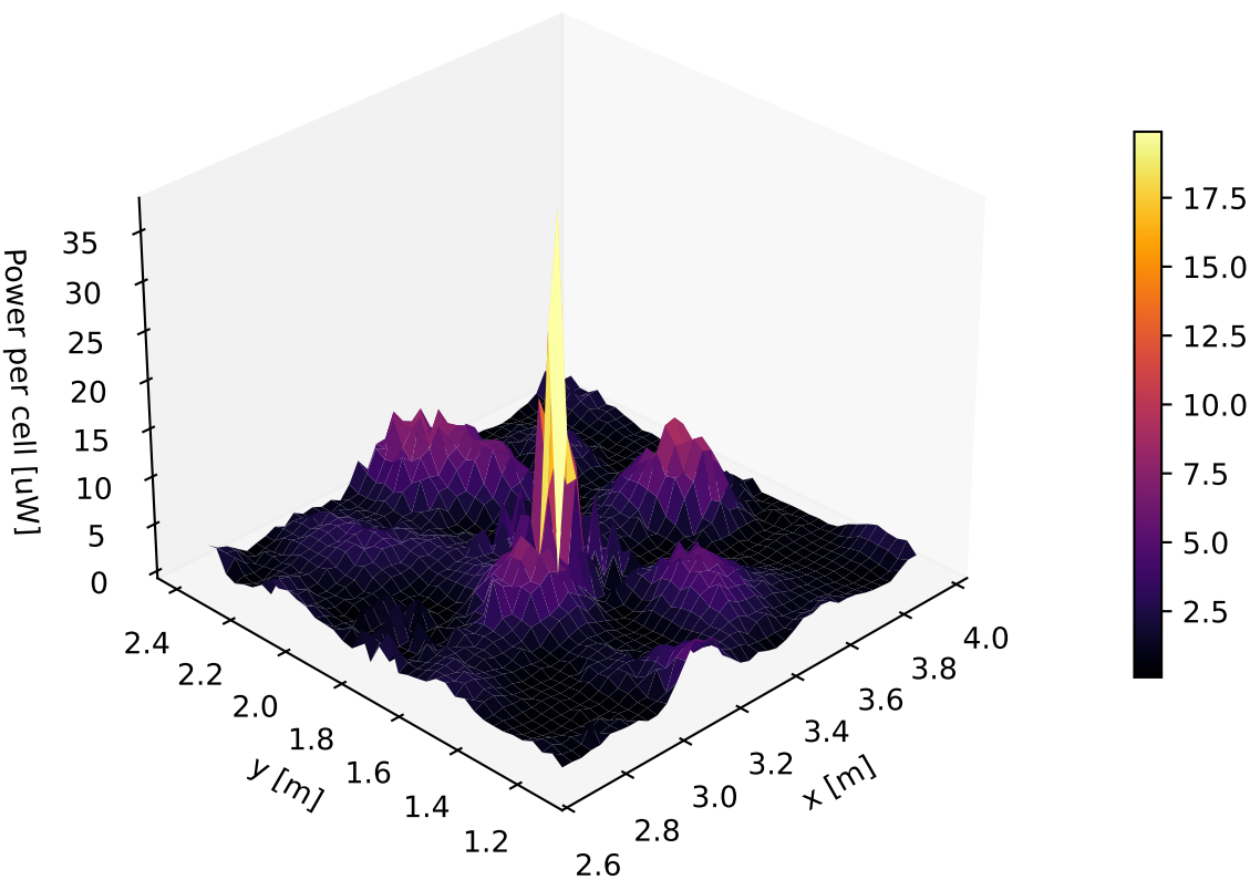
AHMET-Phase2-RF-0 | mean power per cell [ \mu\text{W} ] (3D)
