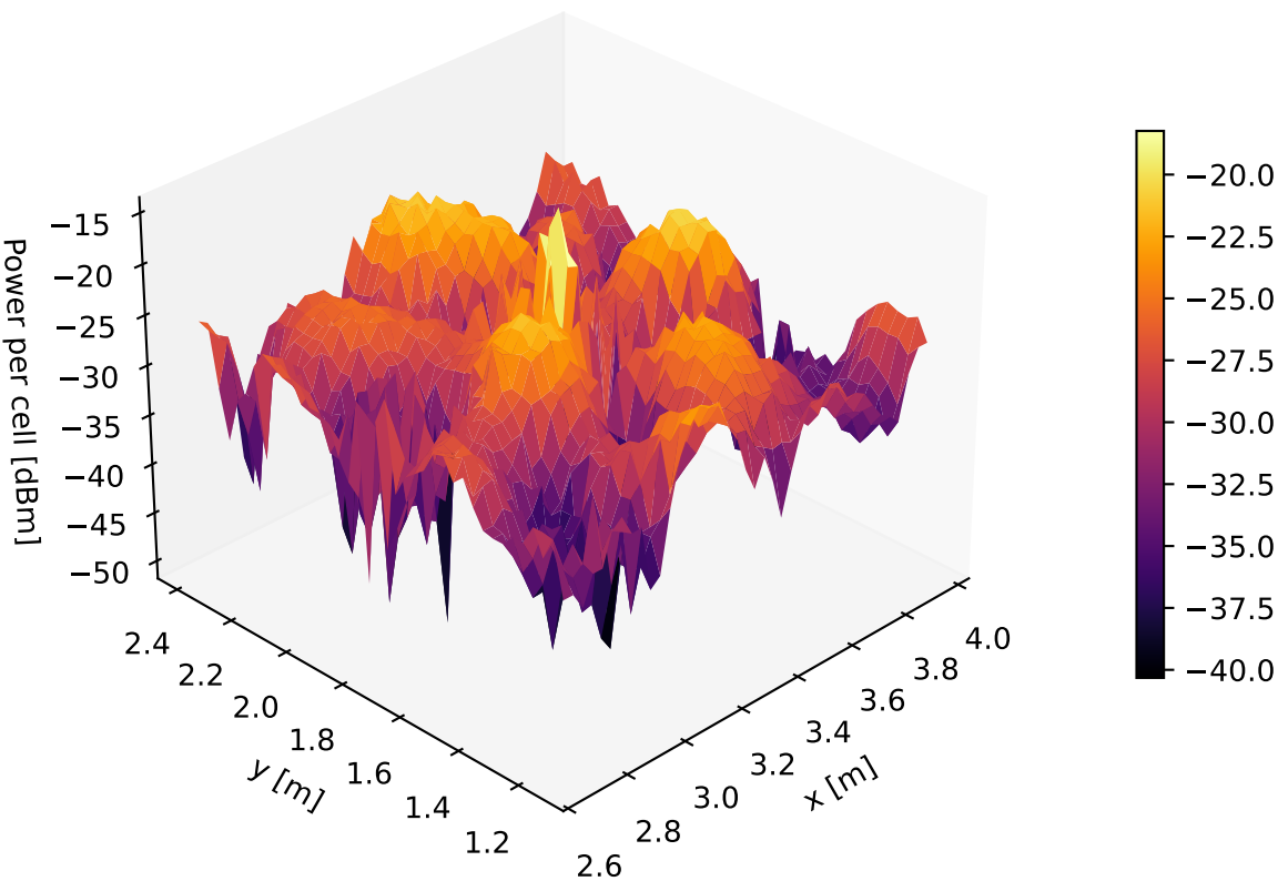
AHMET-Phase2-RF-0 | mean power per cell [dBm] (3D)
