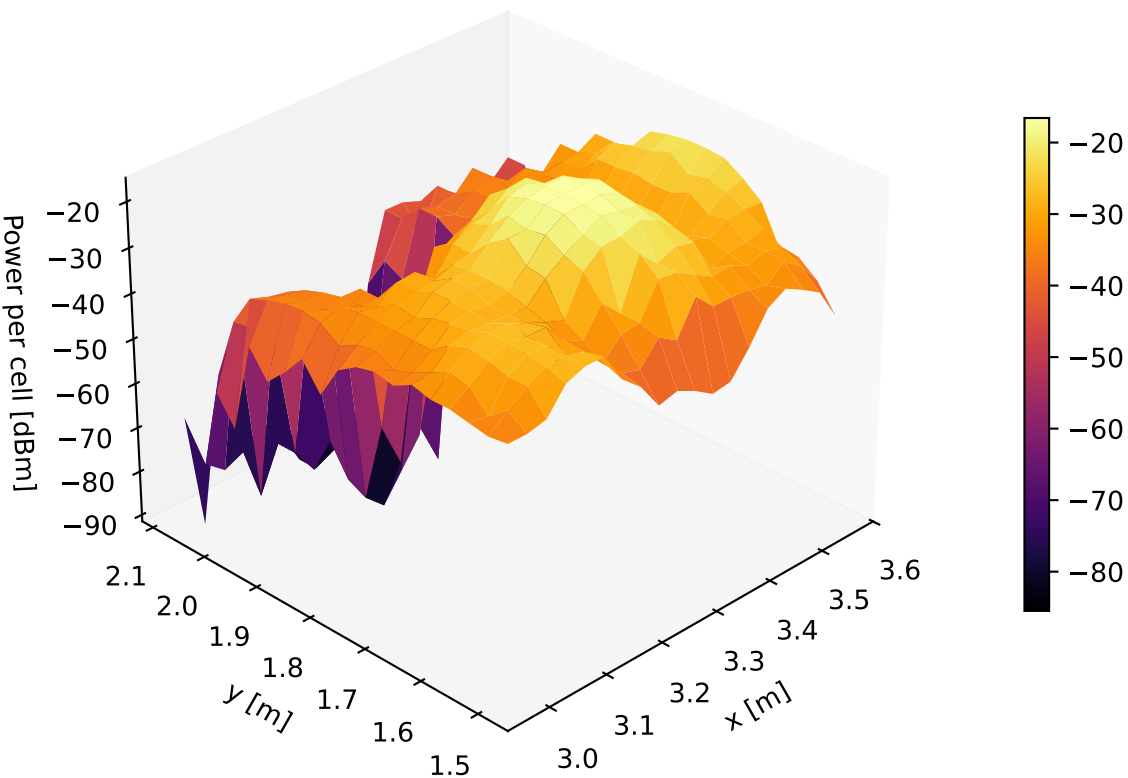
FRIIS-ABS-0 | mean power per cell [dBm] (3D)
