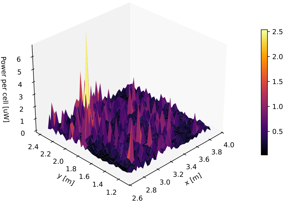
RANDOM-2 | mean power per cell [uW] (3D)
