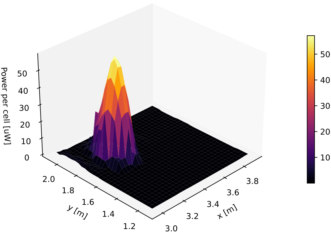
RECI-3 | mean power per cell [uW] (3D)
