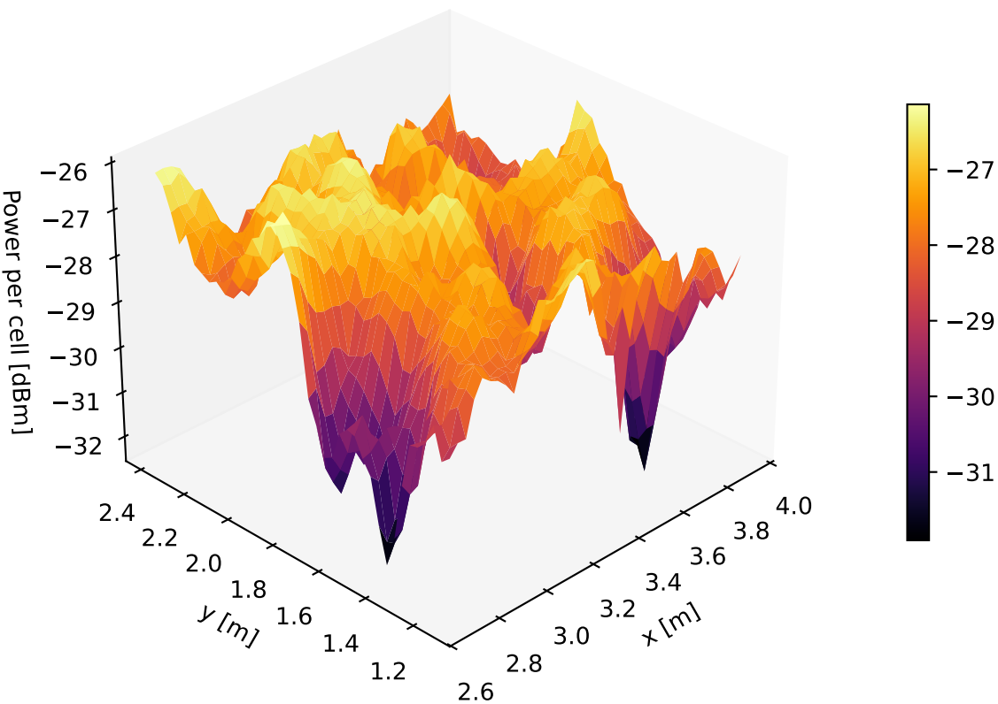
RANDOM | mean power per cell [dBm] (3D)
