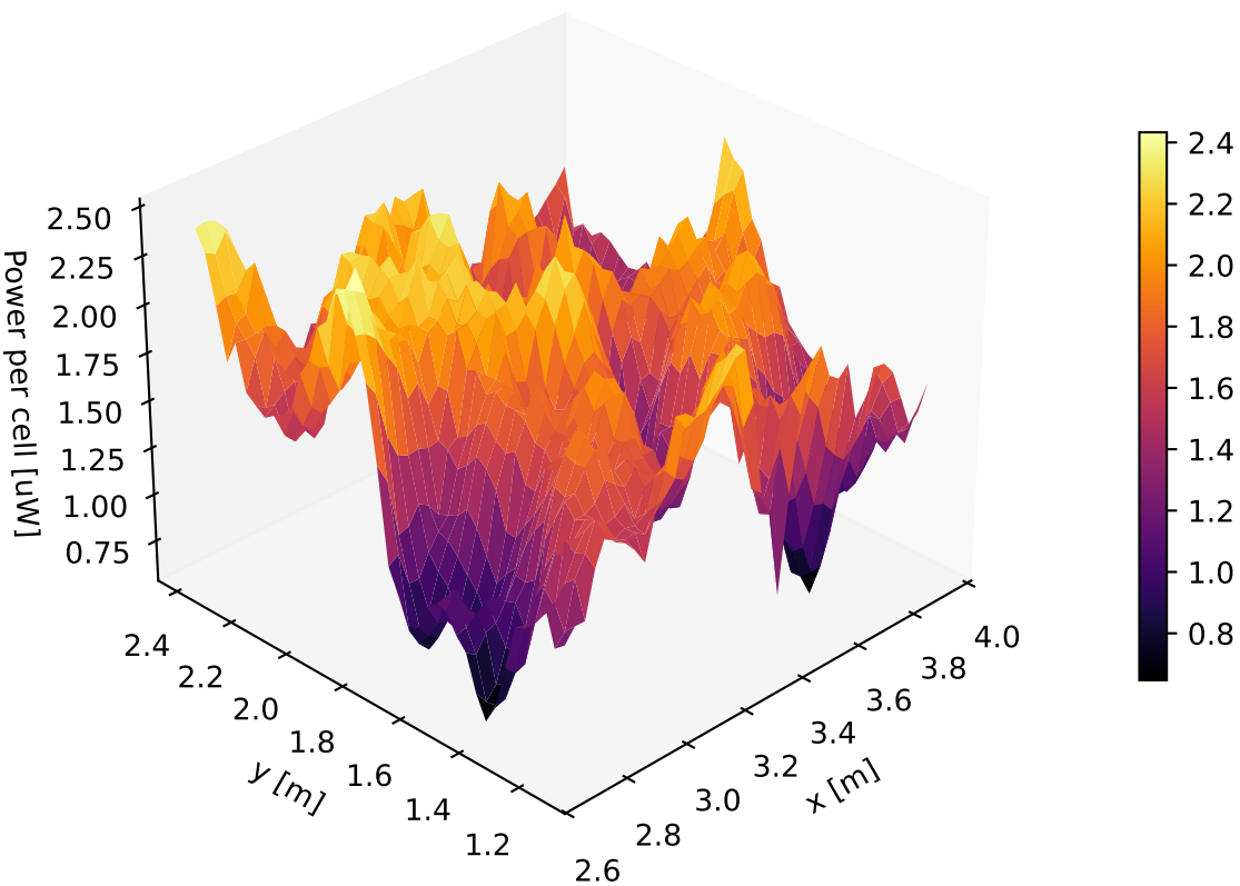
RANDOM | mean power per cell [ \mu\text{W} ] (3D)
