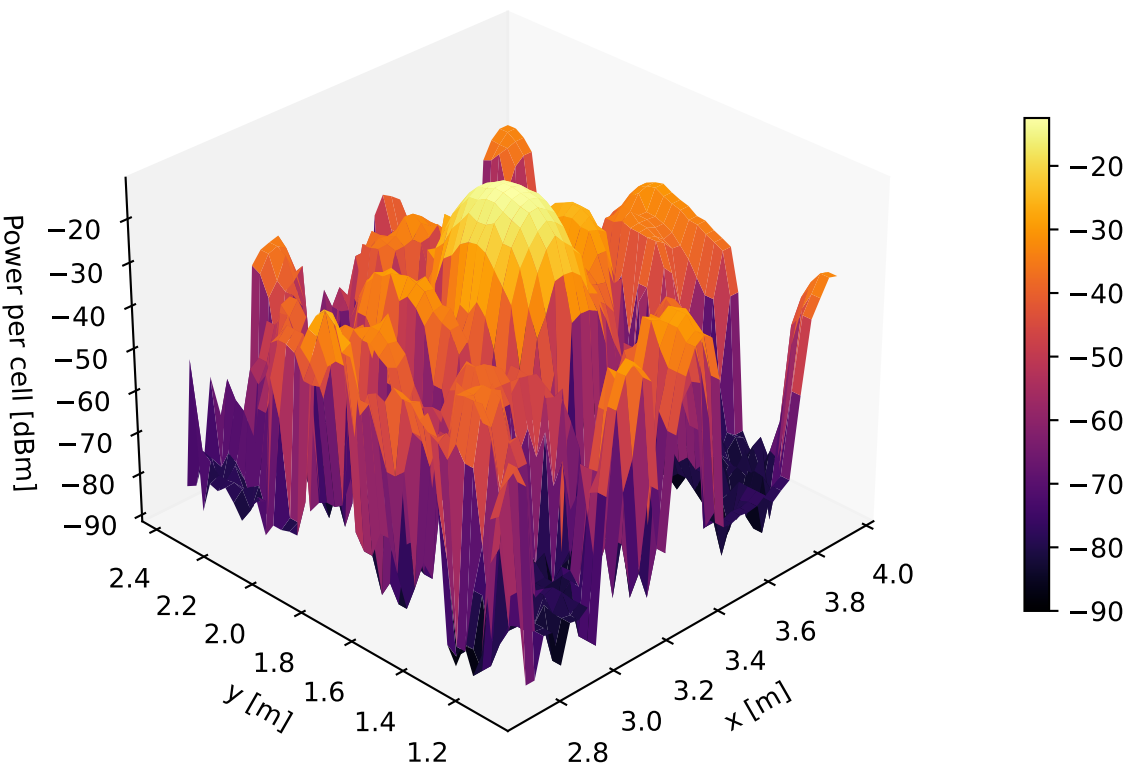
RECI-0 | mean power per cell [dBm] (3D)
