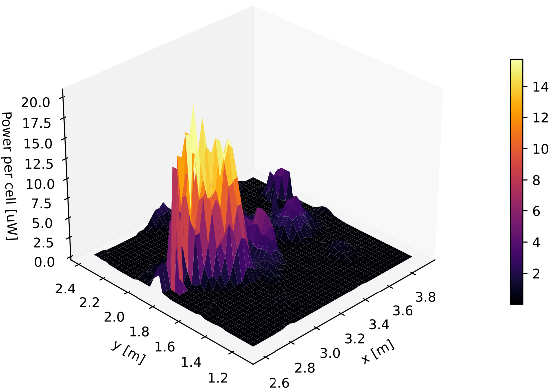
BALL-MAX-20260108095400 | mean power per cell [uW] (3D)
