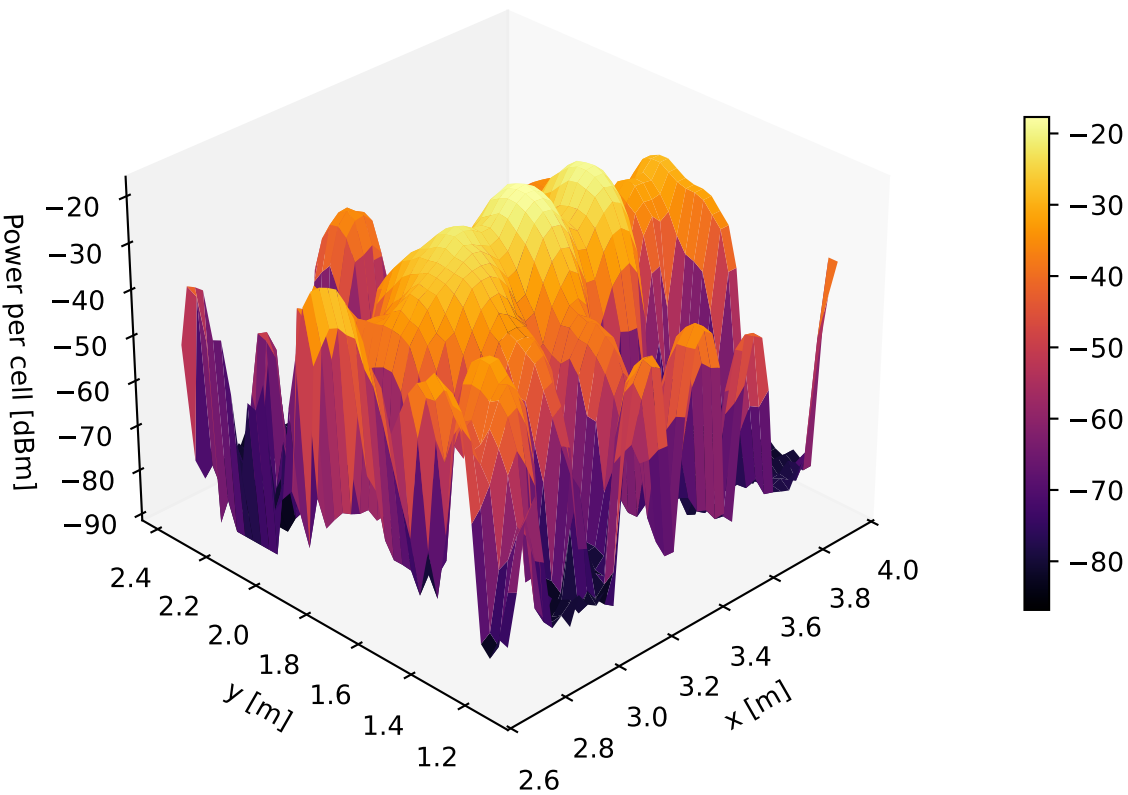
FRIIS-ABS-REFL-0 | mean power per cell [dBm] (3D)
