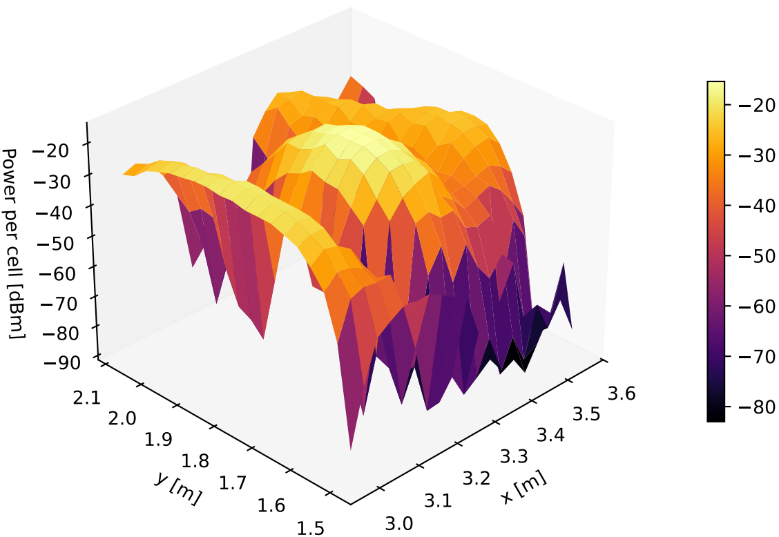
RECI-ABS-0 | mean power per cell [dBm] (3D)
