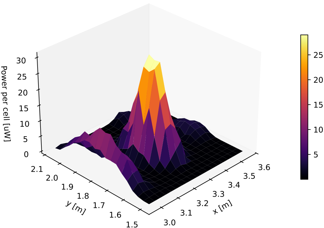
RECI-ABS-0 | mean power per cell [uW] (3D)
