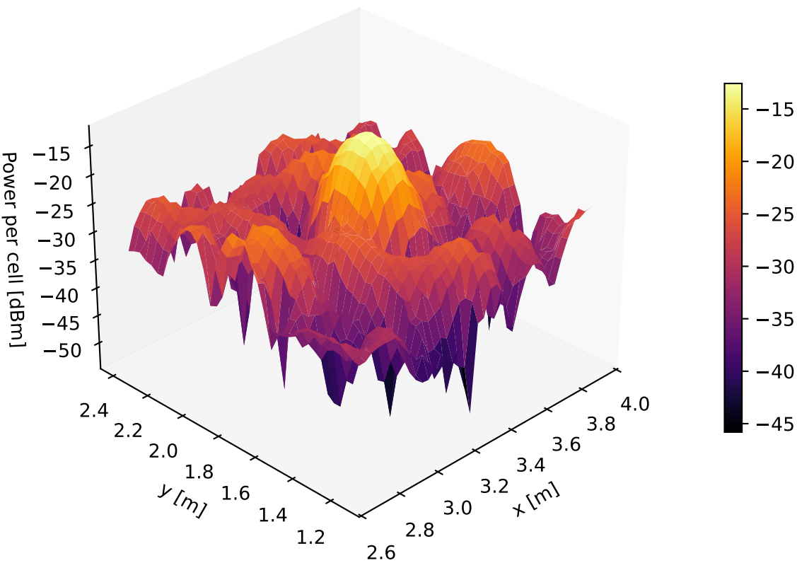
RECI-RF-REFL-0 | mean power per cell [dBm] (3D)
