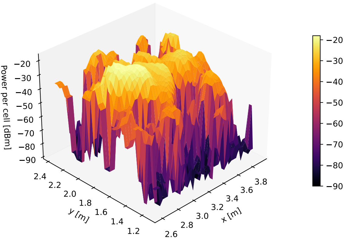
BALL-MAX-20260108095400 | mean power per cell [dBm] (3D)
