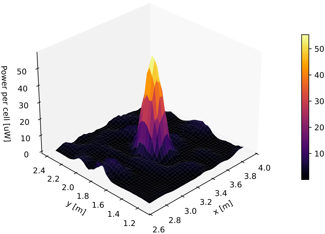
RECI-RF-REFL-0 | mean power per cell [uW] (3D)
