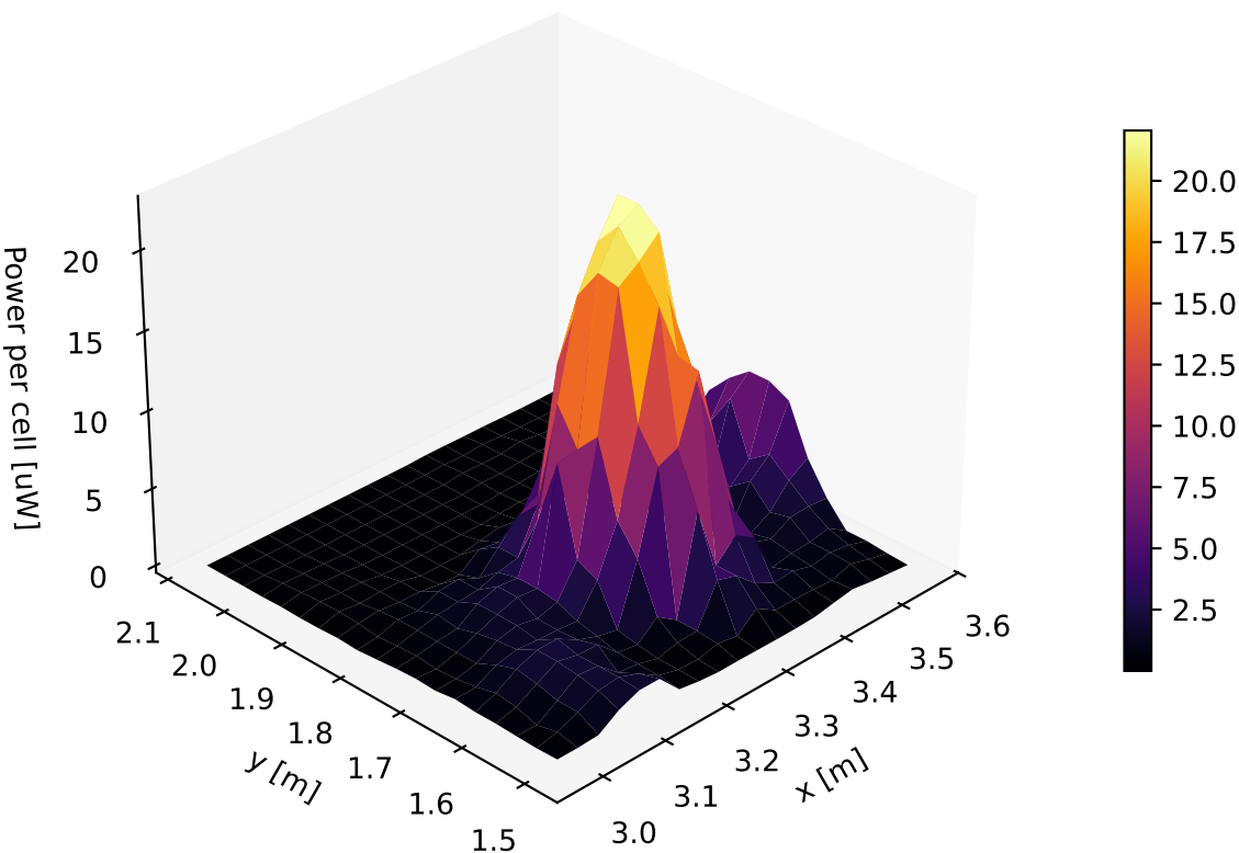
FRIIS-ABS-0 | mean power per cell [uW] (3D)
