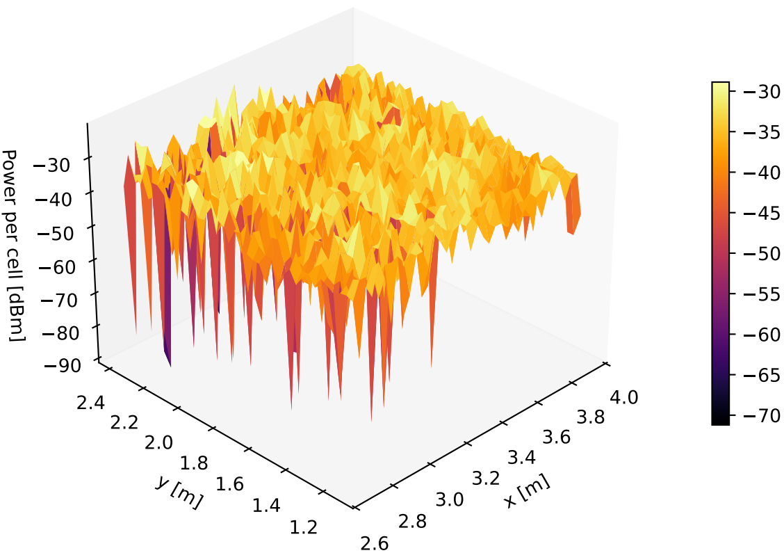
RANDOM-2 | mean power per cell [dBm] (3D)
