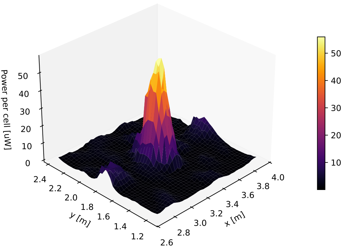
RECI-RF-1 | mean power per cell [ \mu\text{W} ] (3D)
