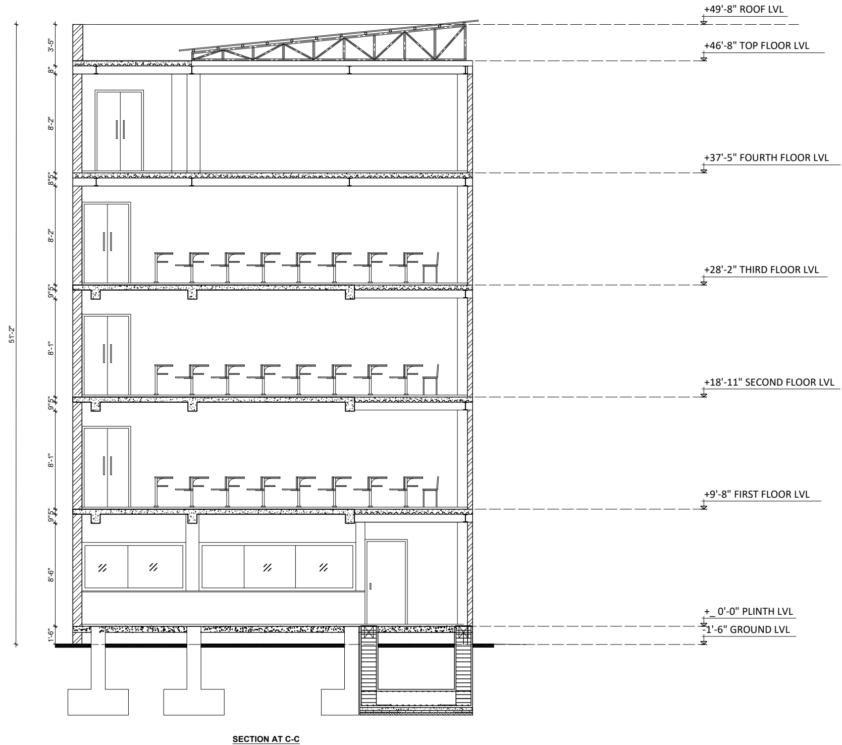
SECTION AT C-C
