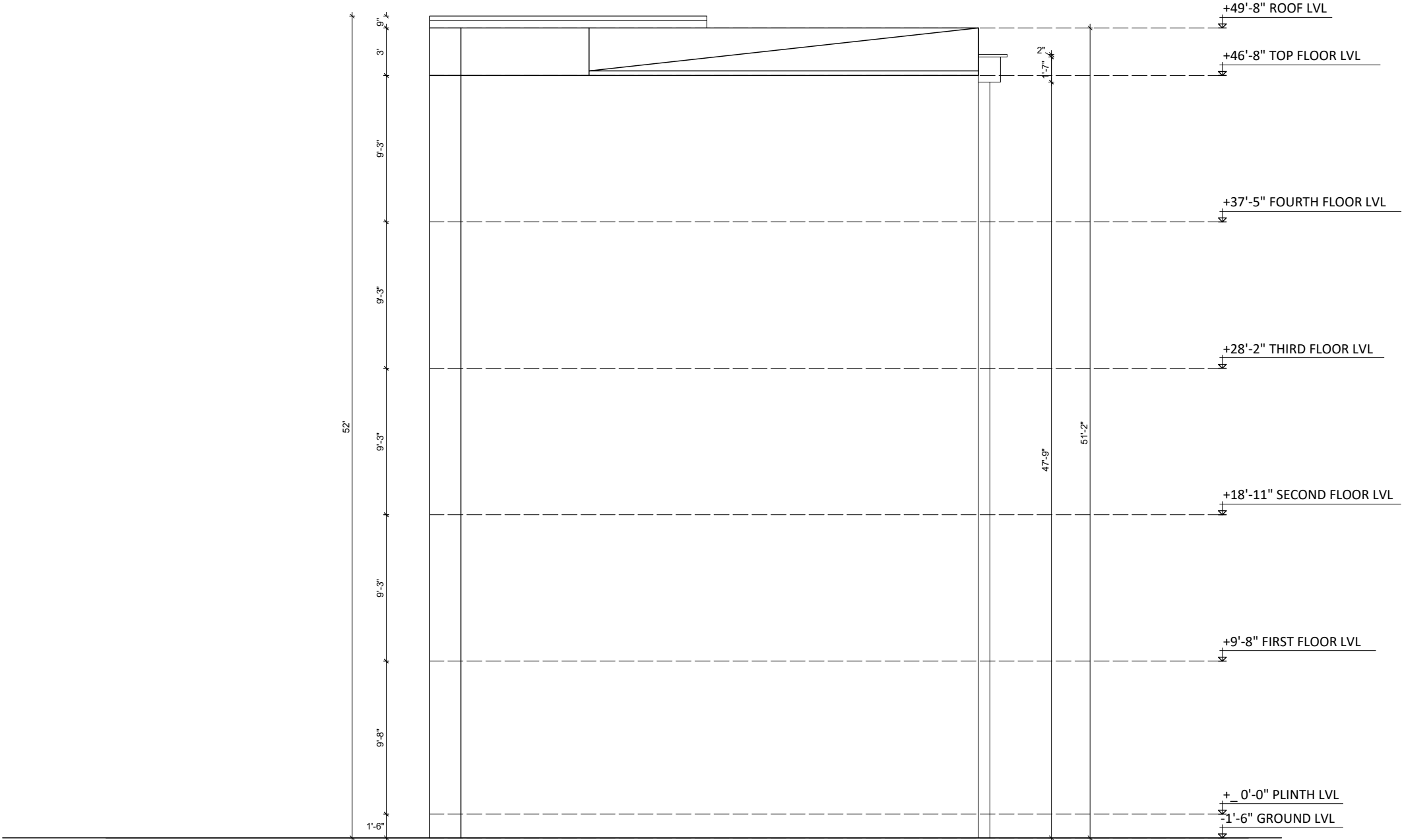
SOUTH ELEVATION
