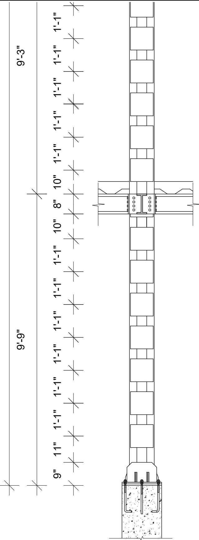
ELEVATION OF COLUMN C1 FRONTAL VIEW
