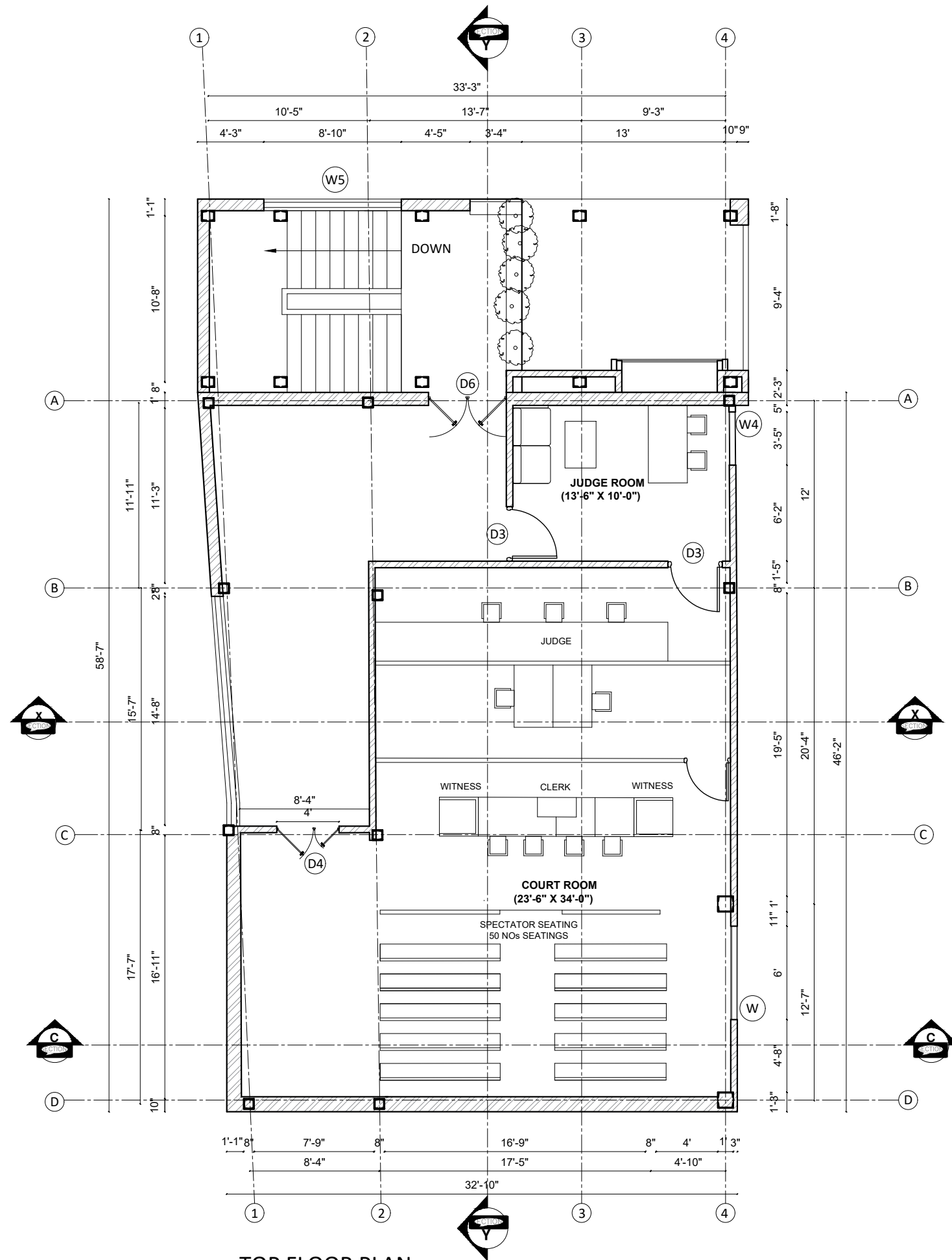
TOP FLOOR PLAN AREA: 1794.02 sq. ft
