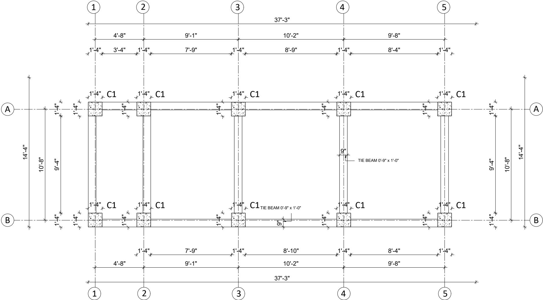
TIE BEAM PLAN
