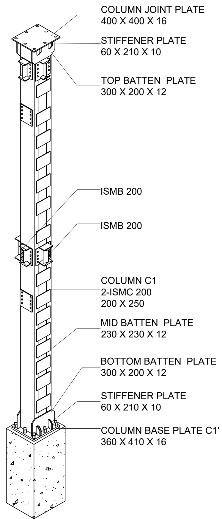
3D- ISOMETRIC VIEW OF COLUMN C1
