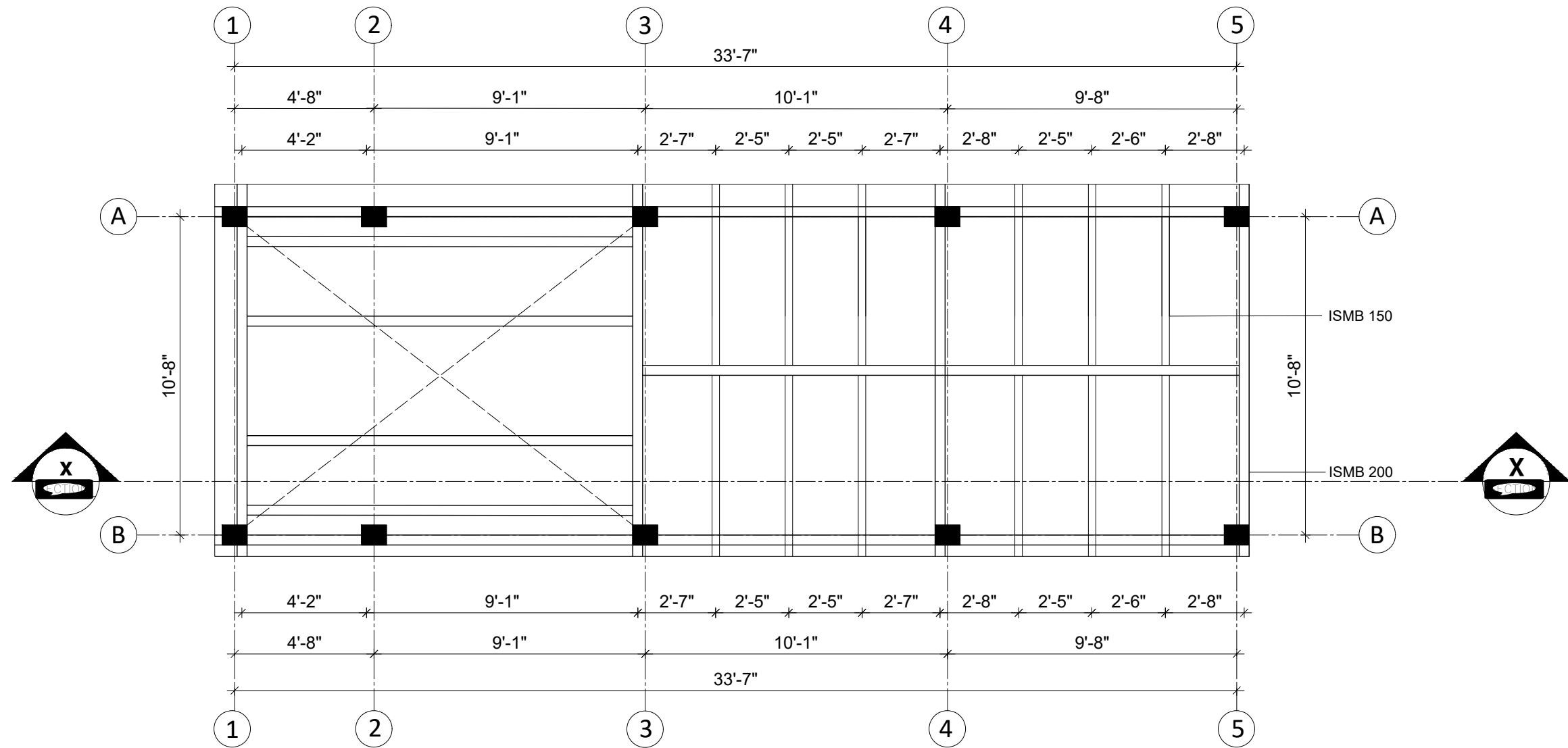
STAIRCASE BEAM PLAN
