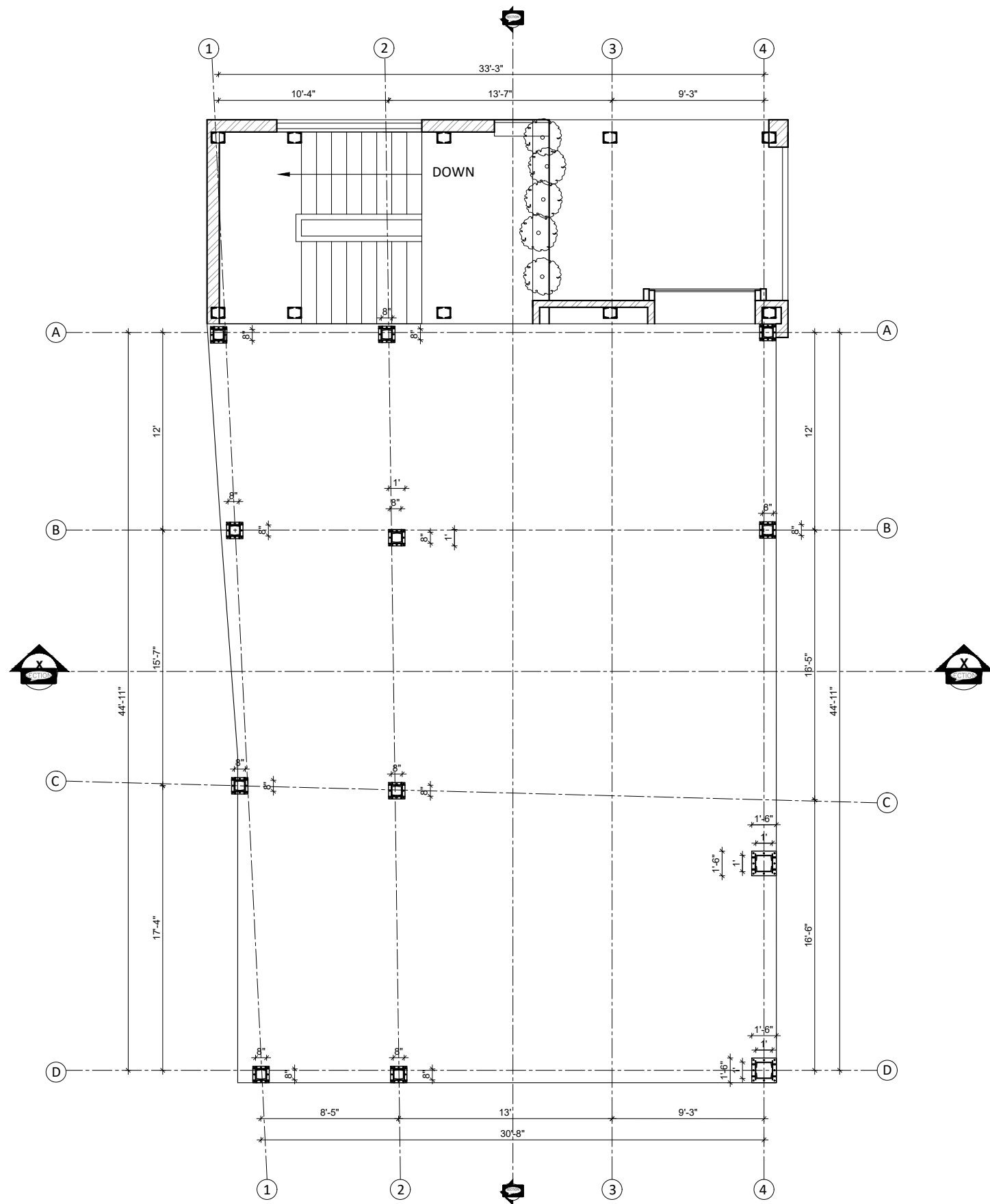
TOP FLOOR COLUMN PLAN
