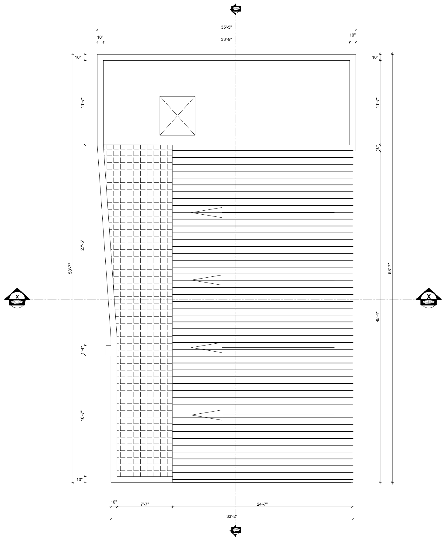
ROOF PLAN
