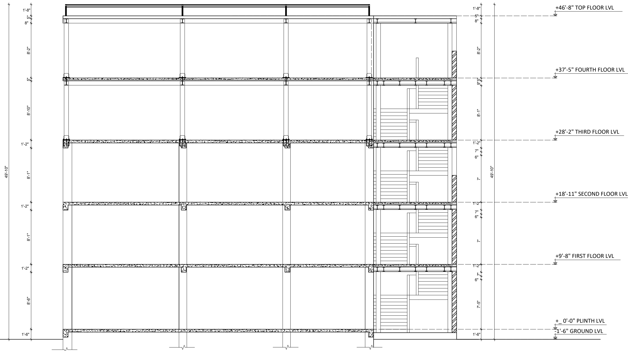
SECTION AT Y-Y
