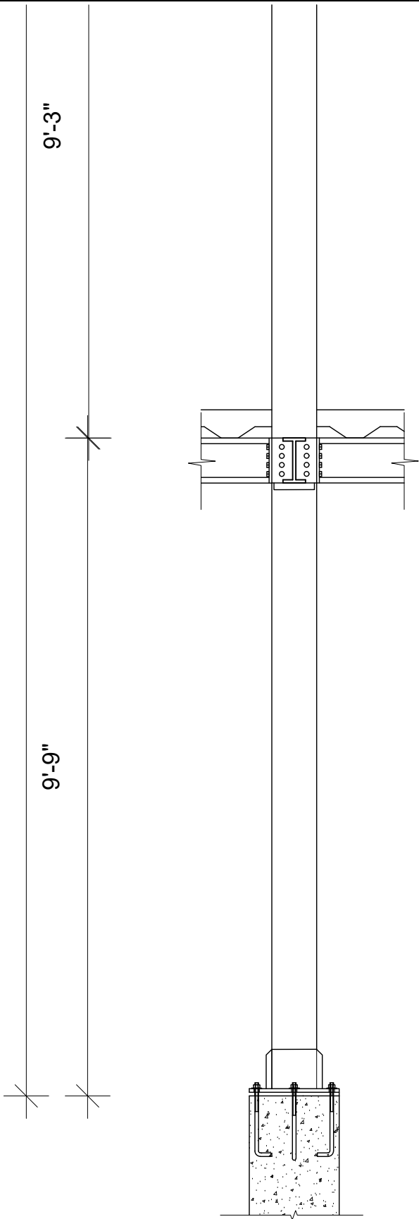
ELEVATION OF COLUMN C1 SIDE VIEW
