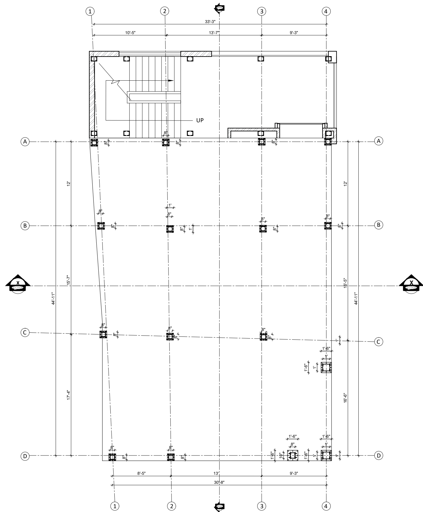
THIRD FLOOR COLUMN PLAN
