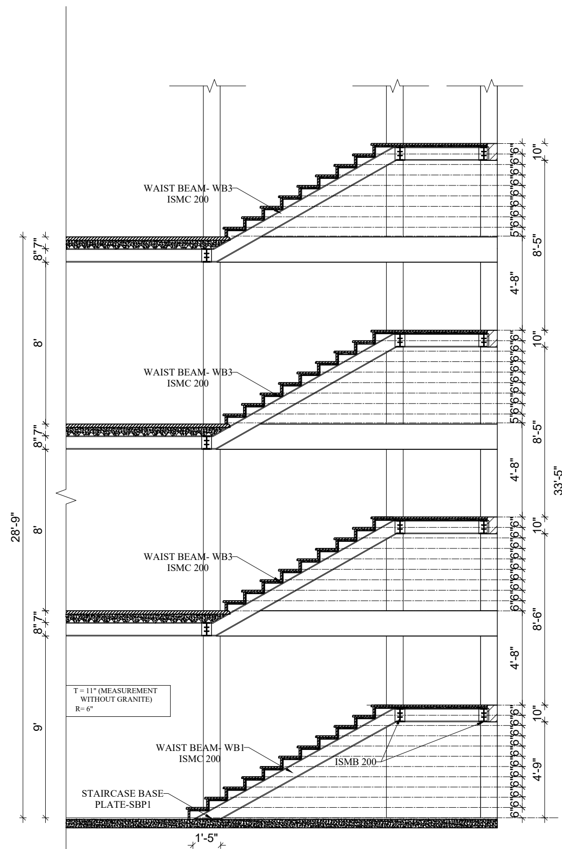
SECTION AT Y-Y
