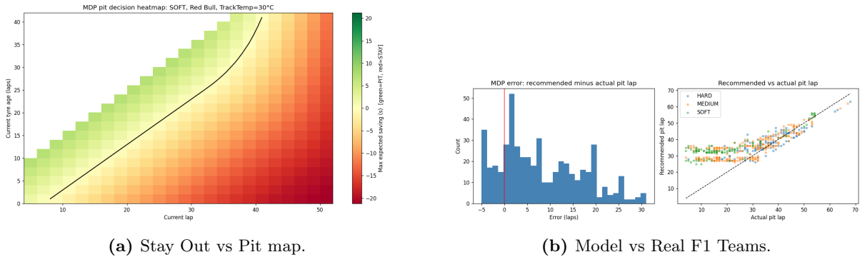
Figure 6: The tool tells the driver when to pit. It stops later than real teams because it does not worry about traffic or other drivers.
