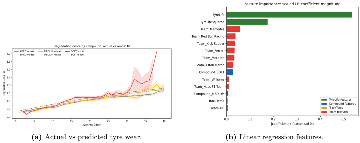
Figure 4: The model correctly shows that softer tyres wear out faster than harder tyres.
