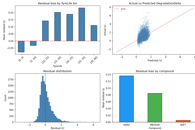
Figure 5: Error checks. The model makes small errors on very old tyres because it misses the sudden cliff where tyres completely lose grip.
