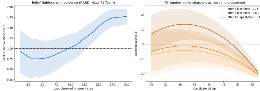
Figure 7: Live updates. As the car drives more laps, the tool becomes more confident about exactly when the tyre will die.
