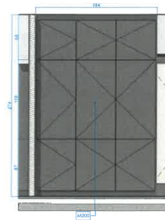
D.2 RECEPTION Cupboard 1:20
