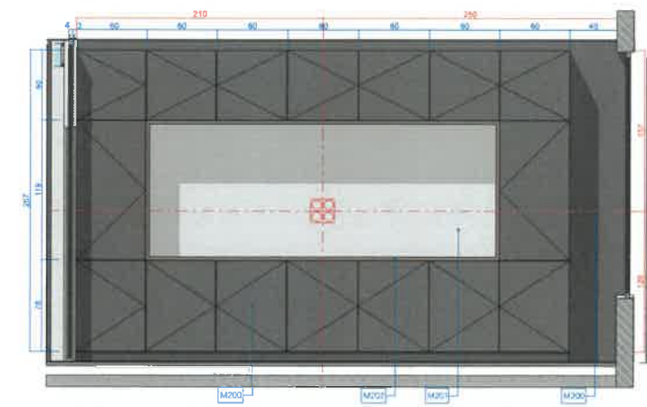
B.1 MEETING ROOM Cupboard 1:20
