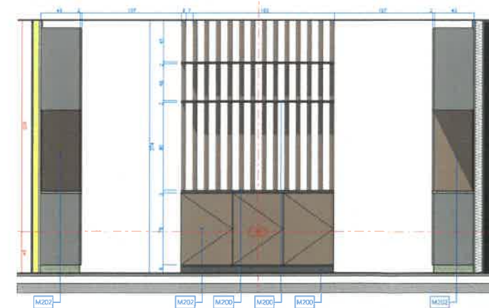
E.3 OPEN SPACE Cupboard 1:20
