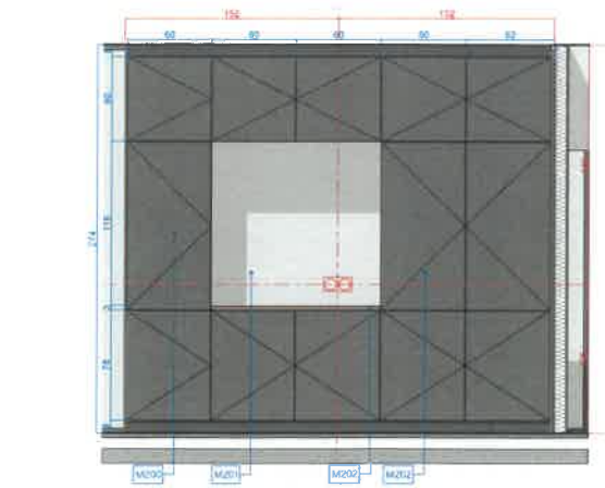
D.1 RECEPTION Cupboard 1:20
