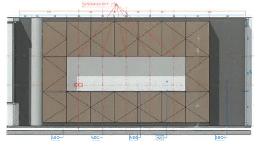
E.1 OPEN SPACE Cupboard 1:20
