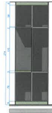
D.3 RECEPTION Cupboard 1:20
