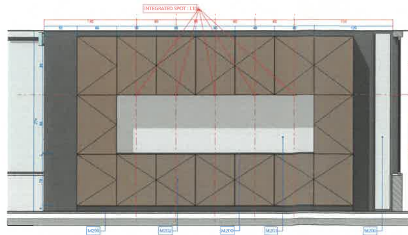
E.2 OPEN SPACE Cupboard 1:20
