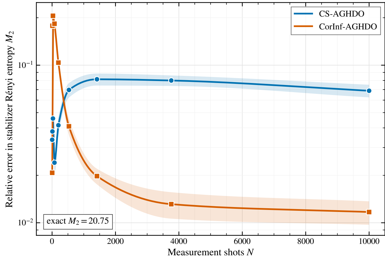
Stabilizer Rényi entropy M_2 : n = 100 , k = 50 , no pilot, 20 repetitions
