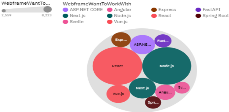
Top 10 WebframeWantToWorkWith
