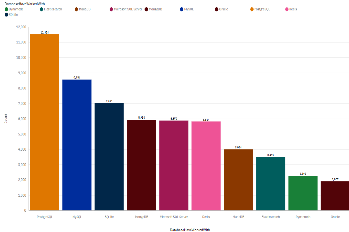
Top 10 DatabaseHaveWorkedWith
