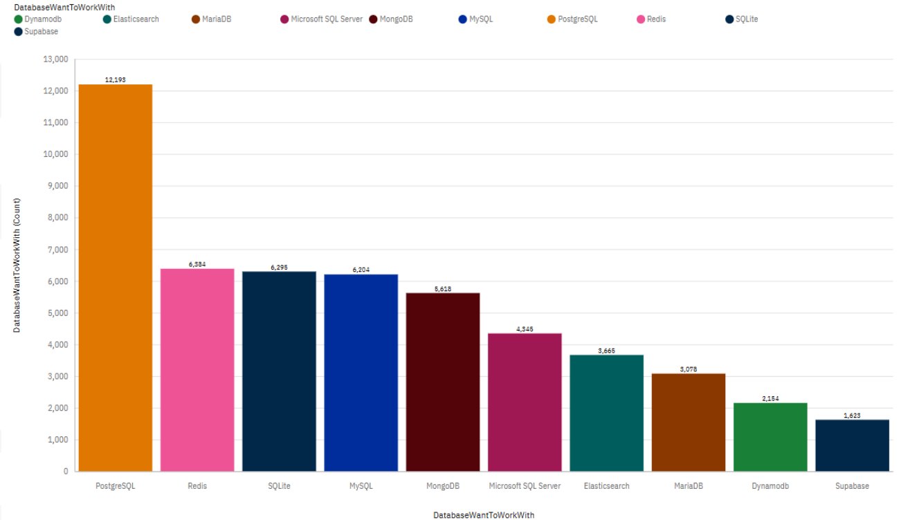
Top 10 DatabaseWantedToWorkWith
