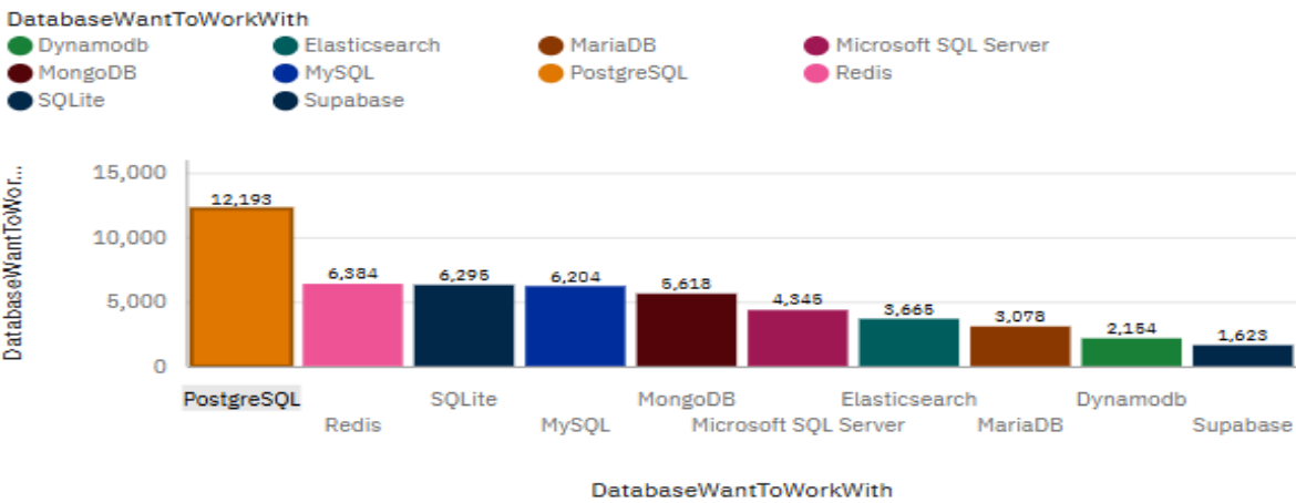
Top 10 DatabaseWantToWorkWith
