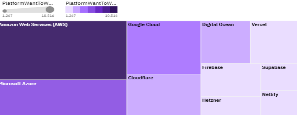
Top 10 PlatformWantToWorkWith
