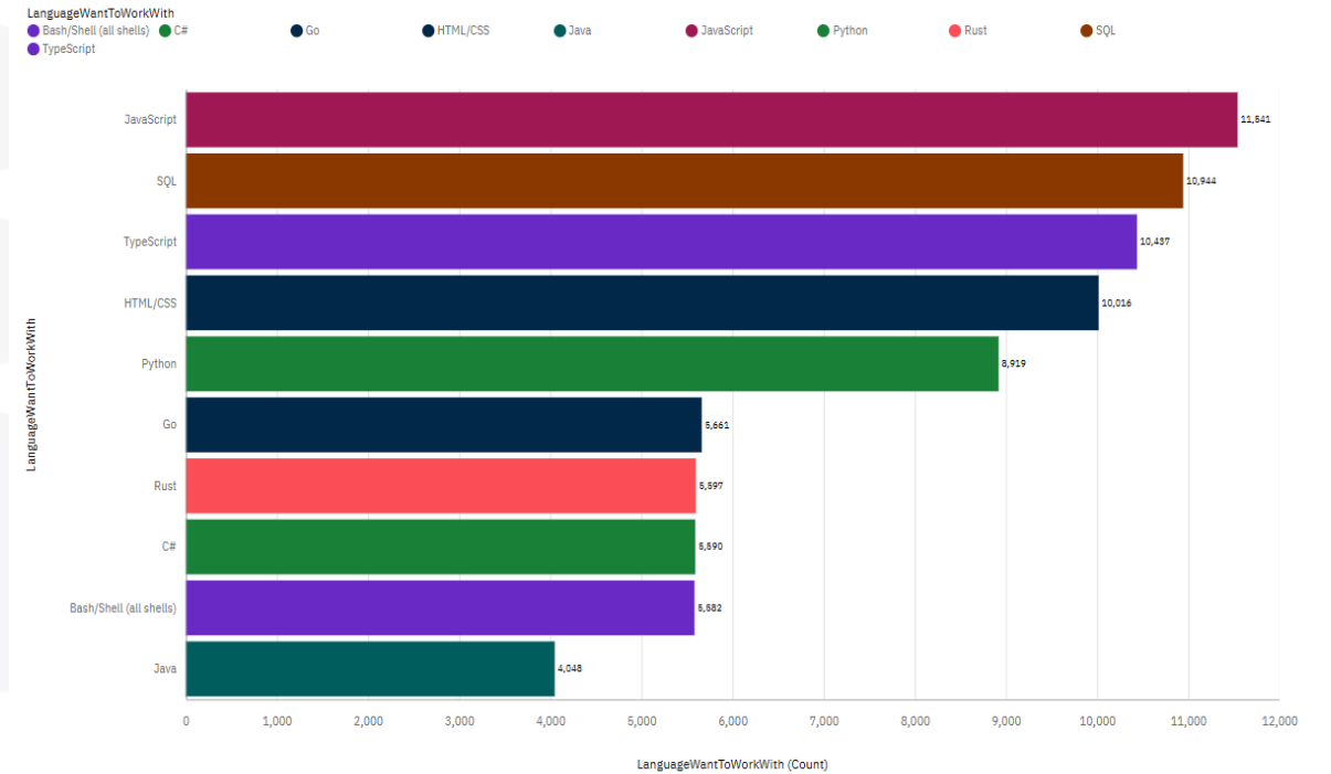
Top 10 LanguageWantToWorkWith
