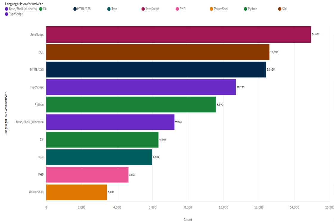
Top 10 LanguageHaveWorkedWith
