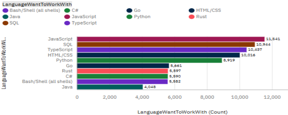
Top 10 LanguageWantToWorkWith
