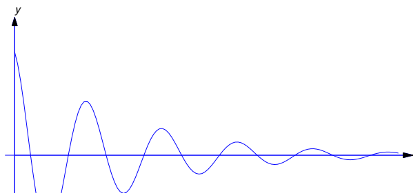
Figure 4.4.13: An oscillatory solution of my'' + cy' + ky = 0
