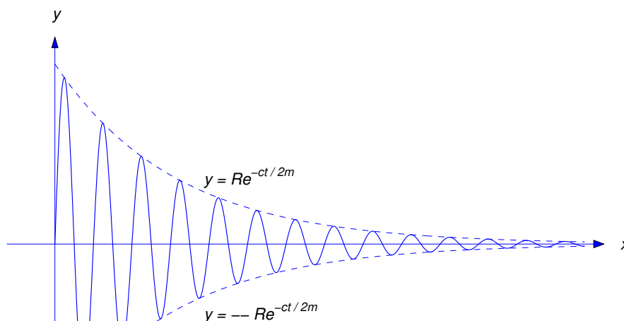
Figure 6.2.1: Underdamped motion
