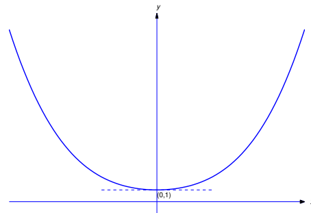
Figure 2.3.4: The unique solution of (2.3.14)
