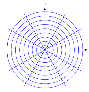
Figure 4.5.10: Curves orthogonal at a point of intersection Figure 4.5.11: Orthogonal families of circles and lines
