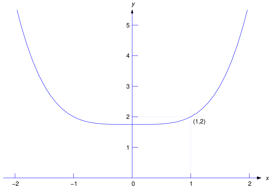
Figure 1.2.2: y = \frac{x^4 + 7}{4}
