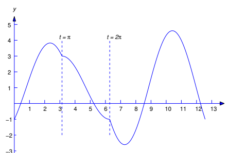
Figure 8.7.5: Graph of (8.7.19)
