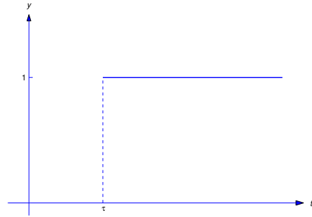
Figure 8.4.2: y = u(t - \tau)
