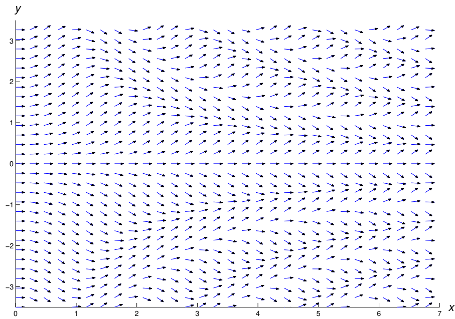
Figure 1.3.7: 7 A direction field for y' = \sin xy
