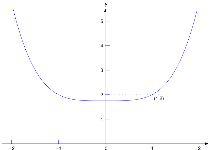
Figure 1.2.2: y = \frac{x^4 + 7}{4}
