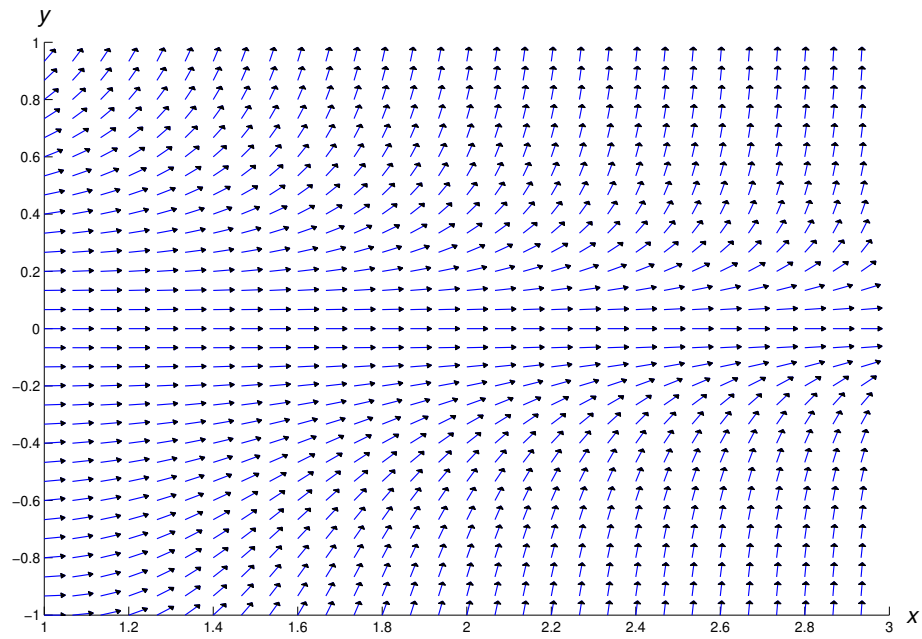
Figure 1.3.7: 10 A direction field for y' = x^3 y^2 + x y^3
