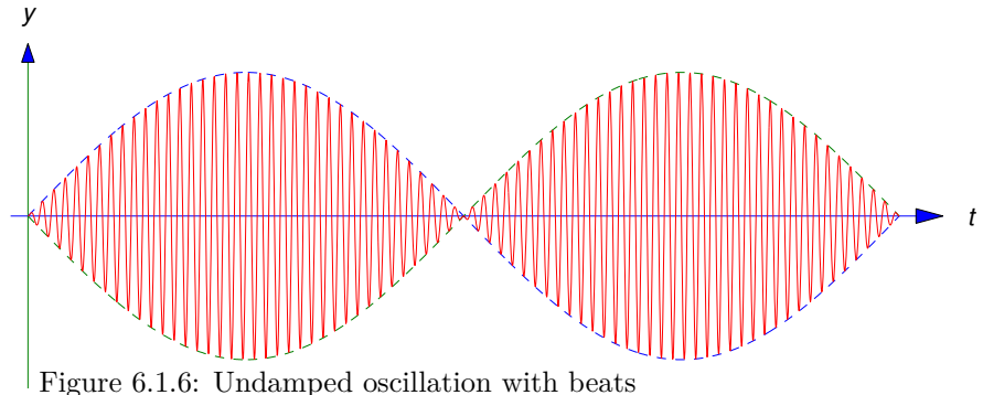
Figure 6.1.6: Undamped oscillation with beats
