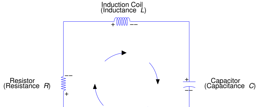
Figure 6.3.1: An RLC circuit
