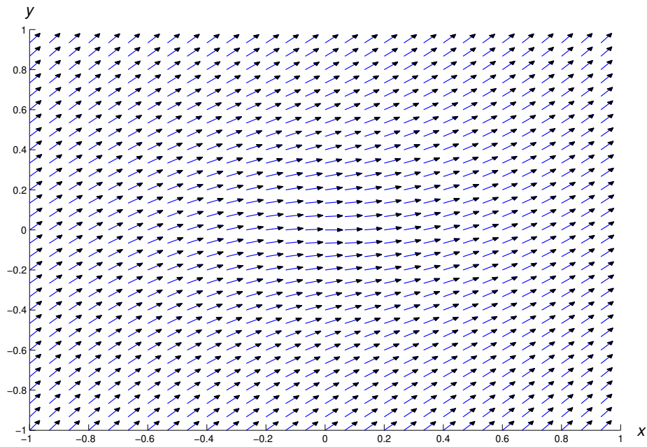
Figure 1.3.7: 6 A direction field for y' = (x^2 + y^2)^{1/2}
