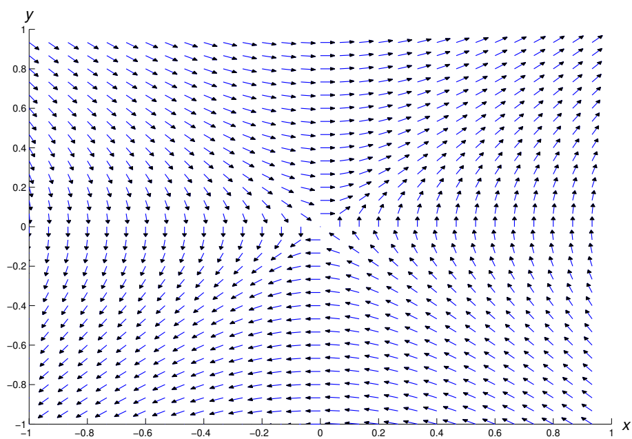
Figure 1.3.7: 1 A direction field for y' = \frac{x}{y}
