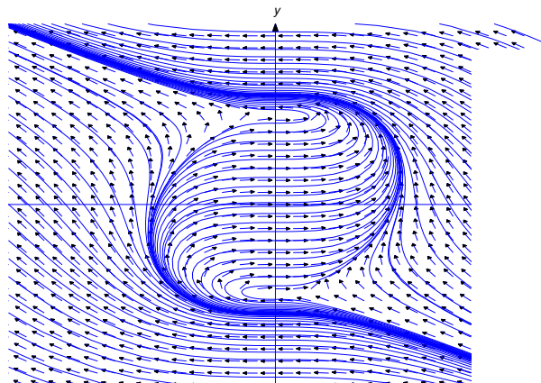
Figure 1.3.6: A direction field and integral curves for y' = \frac{x^2}{-x^2 - y^2}
