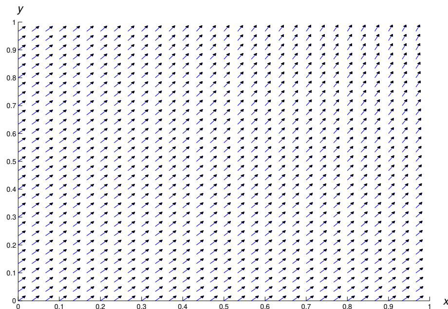
Figure 1.3.7: 8 A direction field for y' = e^{xy}
