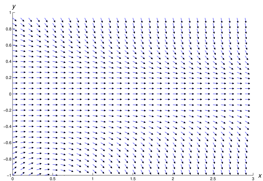
Figure 1.3.7: 5 A direction field for y' = -(2xy^2 + y^3)
