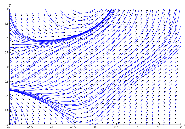
Figure 1.3.3: A direction field and integral
