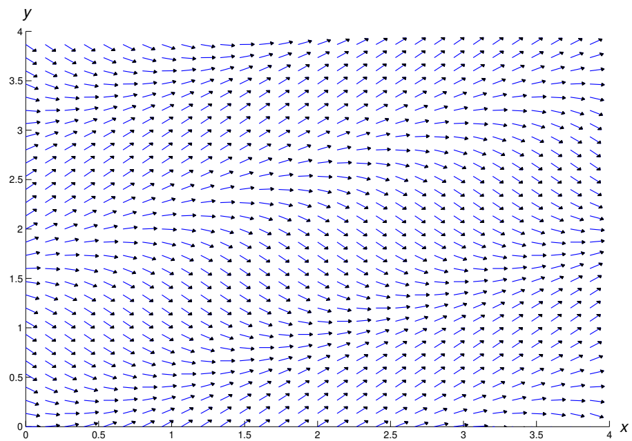
Figure 1.3.7: 11 A direction field for y' = \sin(x - 2y)
