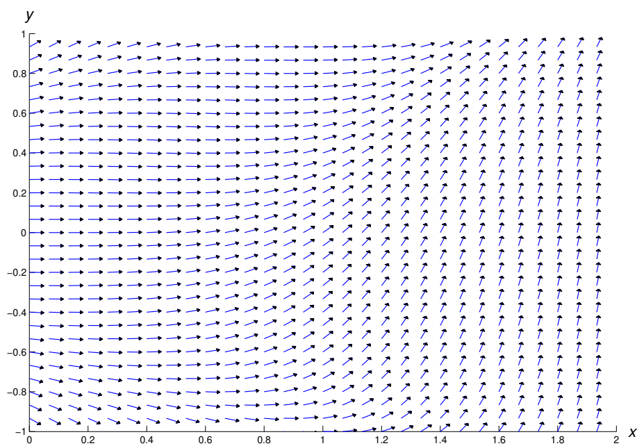
Figure 1.3.7: 9 A direction field for y' = (x - y^2)(x^2 - y)
