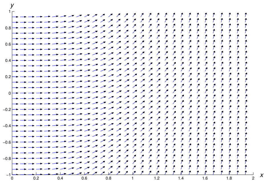
Figure 1.3.7: 3 A direction field for y' = x^2(1+y^2)
