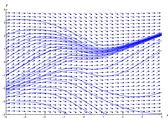
Figure 1.3.2: A direction field and integral
