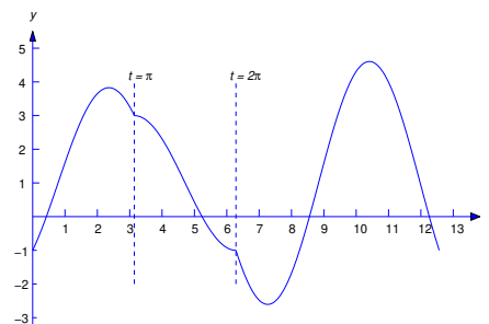
Figure 8.7.5: Graph of (8.7.19)
