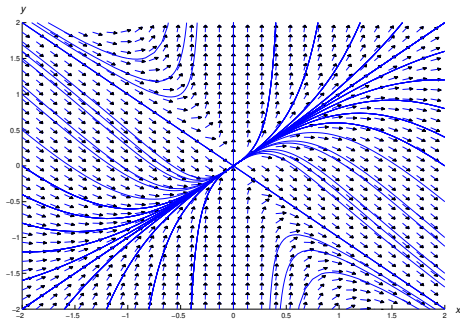
Figure 2.4.3: A direction field and integral curves for x^2 y' = y^2 + xy - x^2 . Therefore
