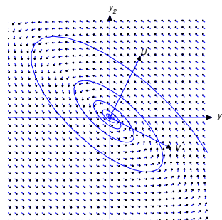
Figure 10.6.6: \alpha < 0 ; shadow trajectory spiraling inward
