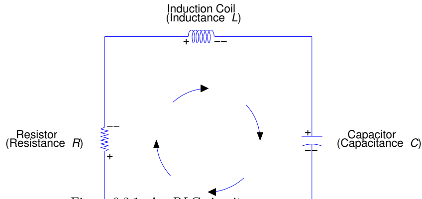
Figure 6.3.1: An RLC circuit
