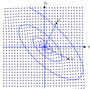
Figure 10.6.4: \alpha > 0 ; shadow trajectory spiraling outward
