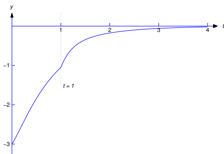
Figure 8.7.4: Graph of (8.7.17)
