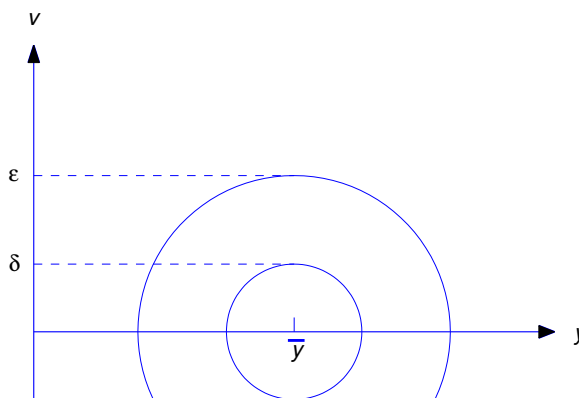
Figure 4.4.1: Stability: if (y_0, v_0) is in the smaller circle then (y(t), v(t)) is in the larger circle for all t > 0
