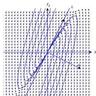
Figure 10.5.5: Negative eigenvalue; motion toward the origin
