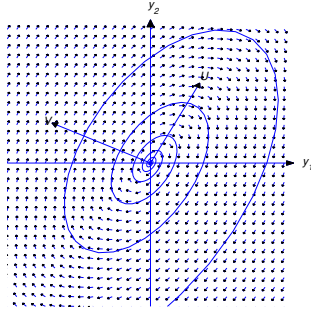
Figure 10.6.3: \alpha > 0 ; shadow trajectory spiraling outward
