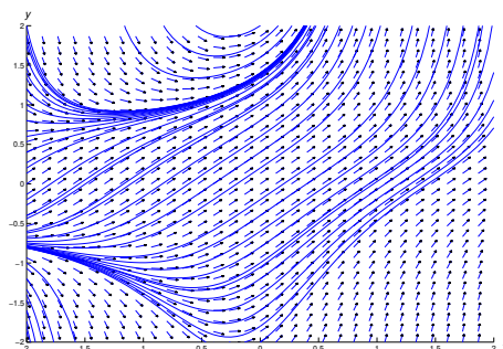
Figure 1.3.3: A direction field and integral
