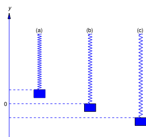
Figure 6.1.1: (a) y > 0 (b) y = 0 , (c) y < 0
