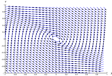
Figure 4.4.11: A typical direction field for my'' + cy' + ky = 0 with 0 < c < c_1 Figure 4.4.12: Figure 4.4.11 with some trajectories added
