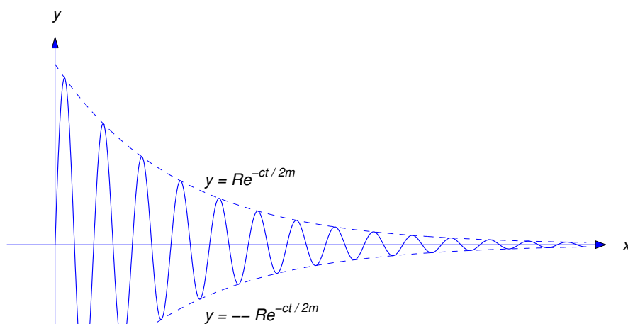
Figure 6.2.1: Underdamped motion
