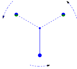
Figure 4.4.8: The whirling undamped pendulum
