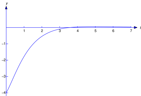
Figure 8.3.1: y = \frac{4}{3}e^{-t/2} - 8e^{-t} + \frac{8}{3}e^{-2t}
