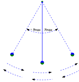
Figure 4.4.9: The oscillating undamped pendulum
