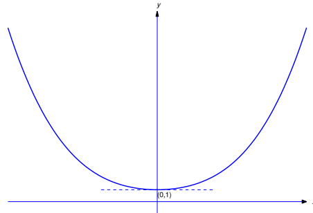
Figure 2.3.4: The unique solution of (2.3.14)
