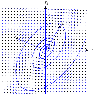
Figure 10.6.5: \alpha < 0 ; shadow trajectory spiraling inward
