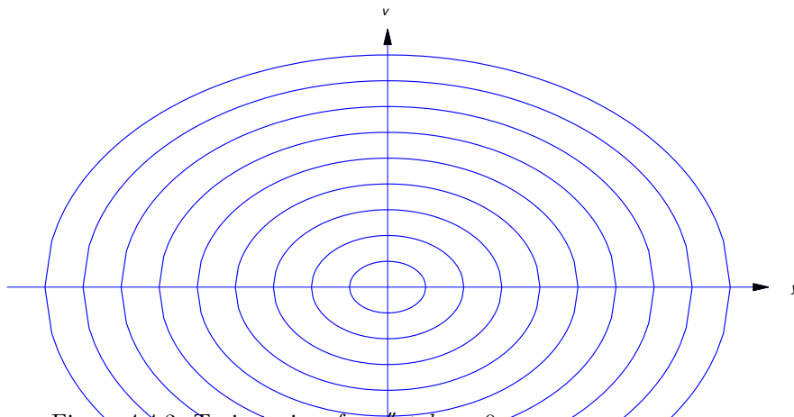
Figure 4.4.3: Trajectories of my'' + ky = 0
