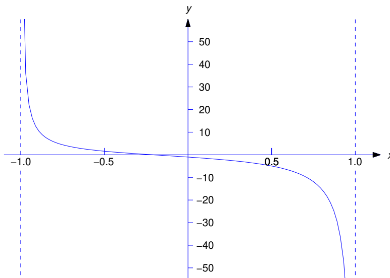
Figure 5.7.1: y = \frac{2 \ln(x+1)}{x-1} + \frac{3x+1}{x^2-1}
