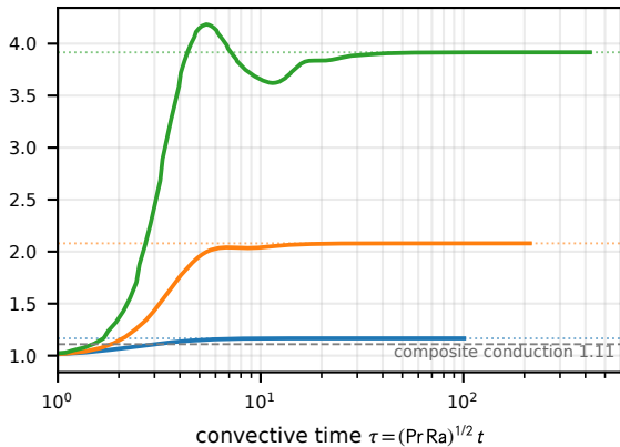
k_r=100 (near-isothermal partition)
