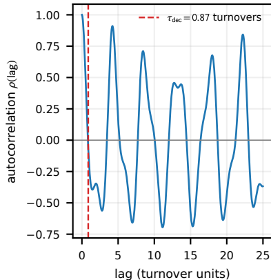
Nu autocorrelation: N_{\text{indep}} \approx 4120
