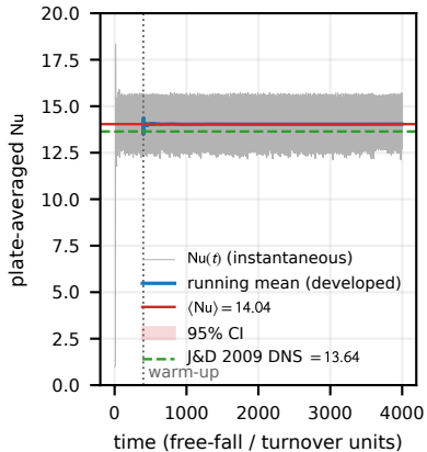
RBC Ra = 10^7 , \Gamma = 2 , Pr = 0.71 (h128)
