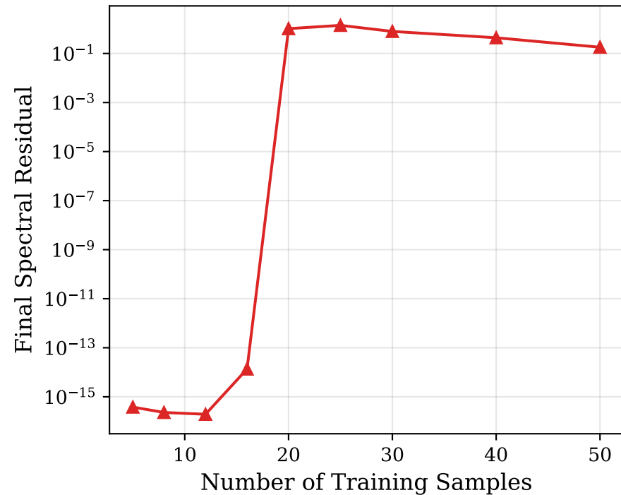
Convergence Residual vs Training Size
