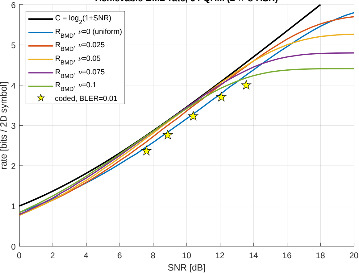
Achievable BMD rate, 64-QAM ( 2 \times 8 -ASK)
