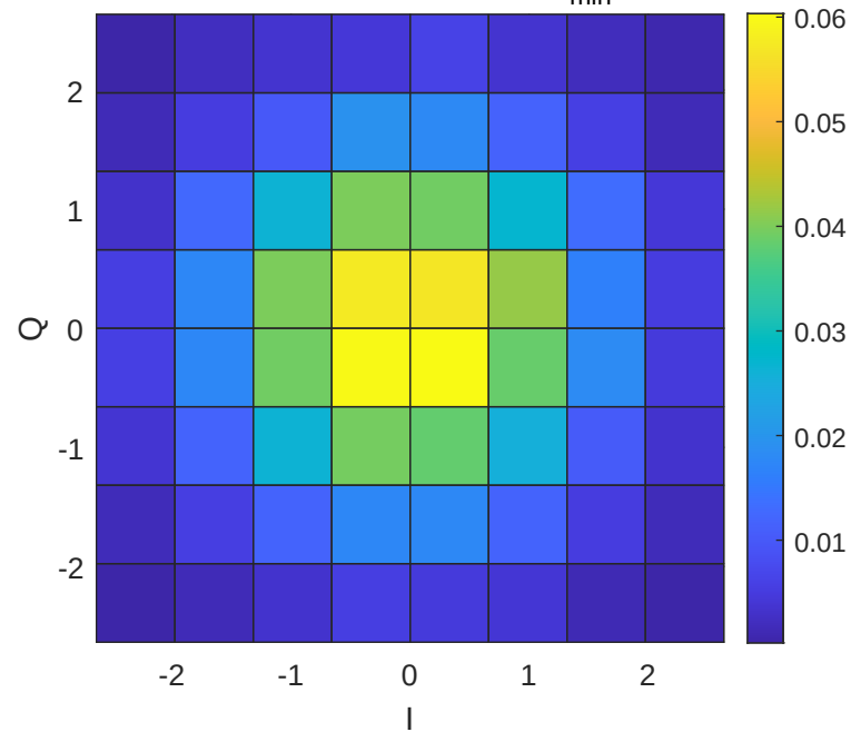
(b) P(x_I, x_Q)
