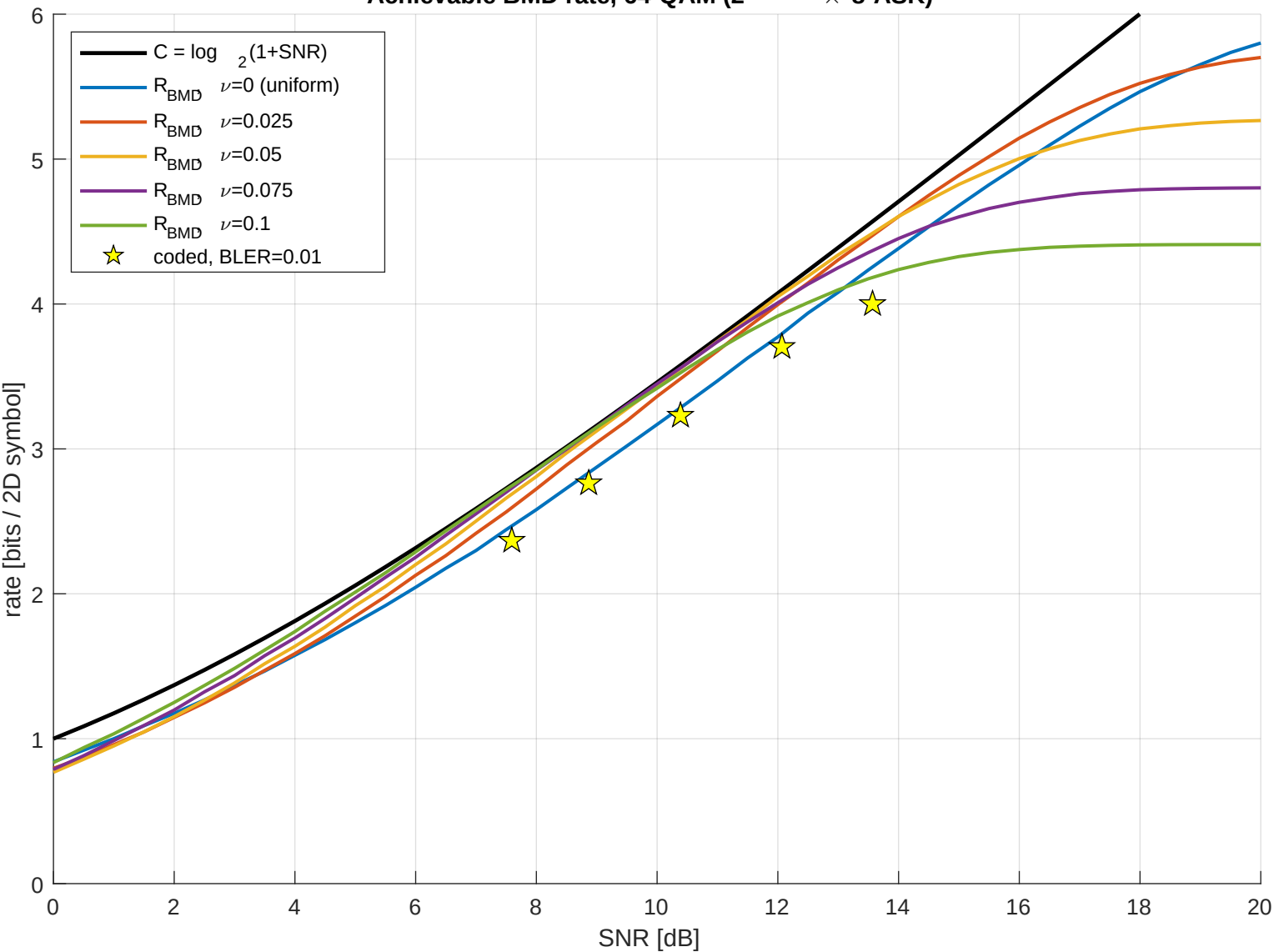
Achievable BMD rate, 64-QAM (2 × 8-ASK)
