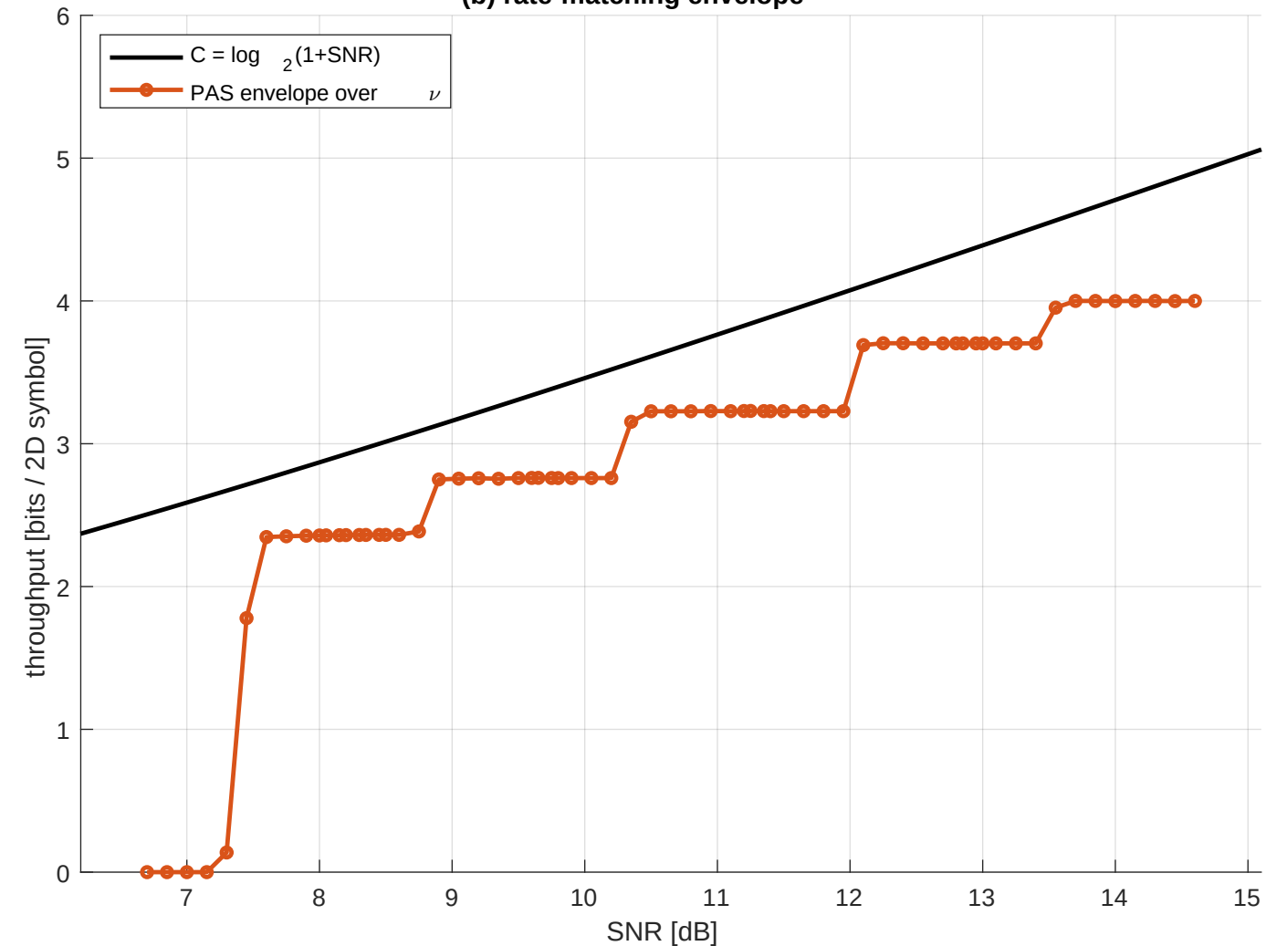
(b) rate-matching envelope
