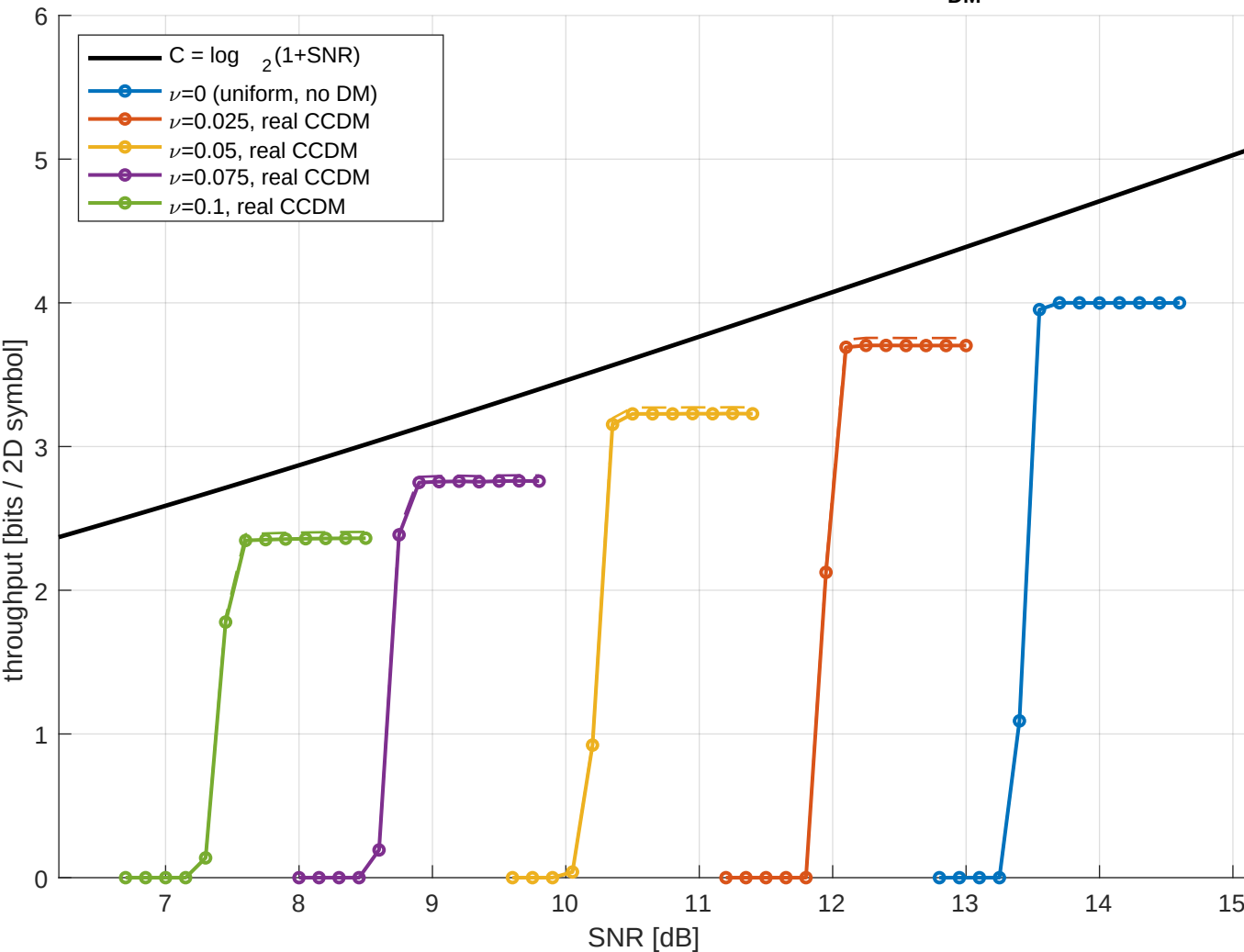
(a) per- \nu throughput (dashed = loss-free, n_{DM}=540 )
