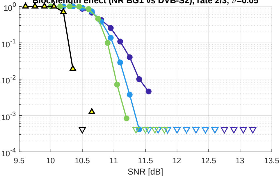
Blocklength effect (NR BG1 vs DVB-S2), rate 2/3, \nu=0.05
