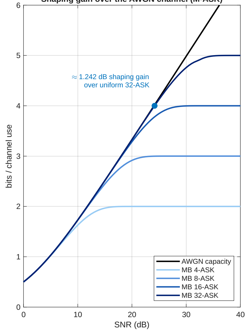
Shaping gain over the AWGN channel (M-ASK)
