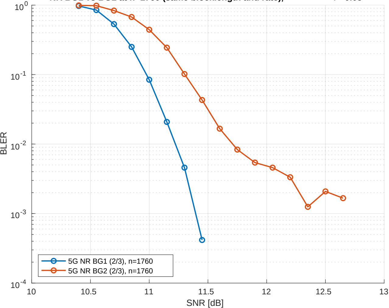
NR BG1 vs BG2 at n=1760 (same blocklength and rate),
