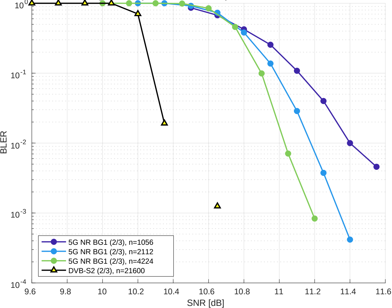
Blocklength effect (NR BG1 vs DVB-S2), rate 2/3,
