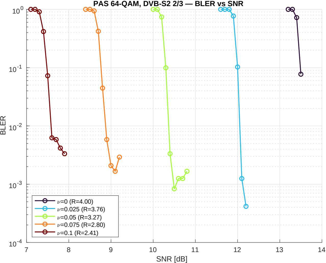
PAS 64-QAM, DVB-S2 2/3 — BLER vs SNR
