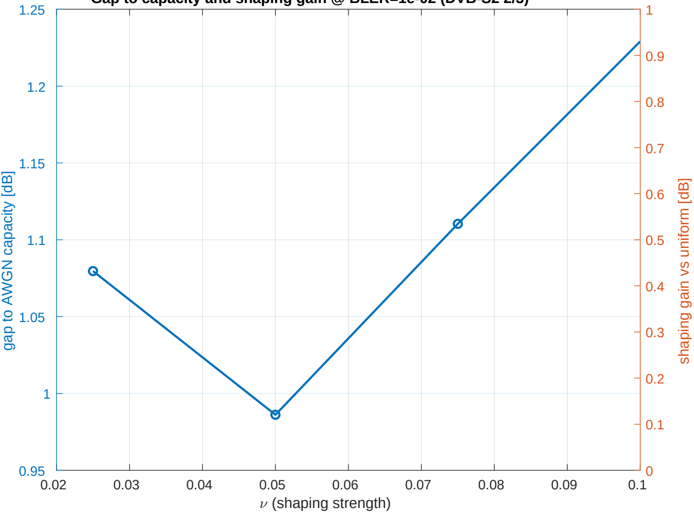
Gap to capacity and shaping gain @ BLER=1e-02 (DVB-S2 2/3)
