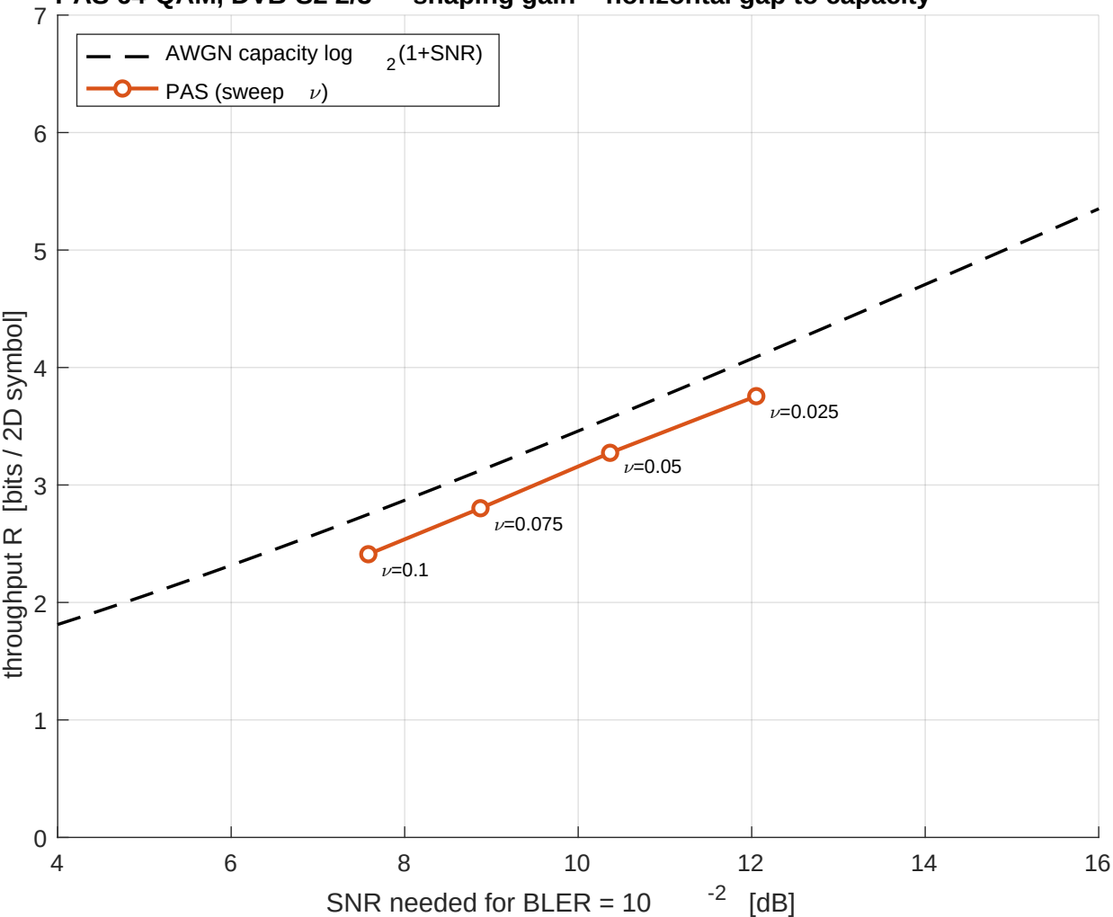
PAS 64-QAM, DVB-S2 2/3 — shaping gain = horizontal gap to capacity
