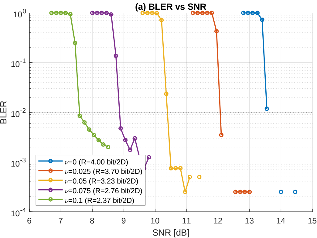
Shaping sweep, DVB-S2 (2/3), 64-QAM
