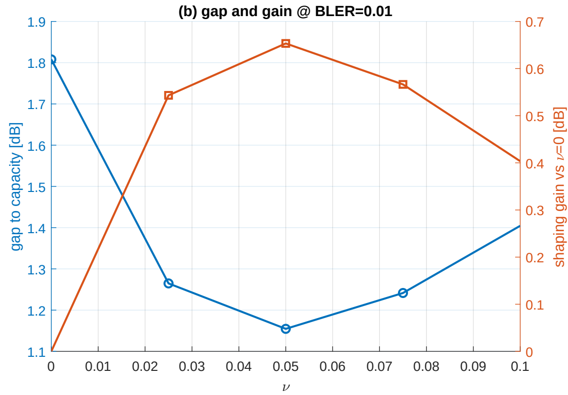
Shaping sweep, DVB-S2 (2/3), 64-QAM
