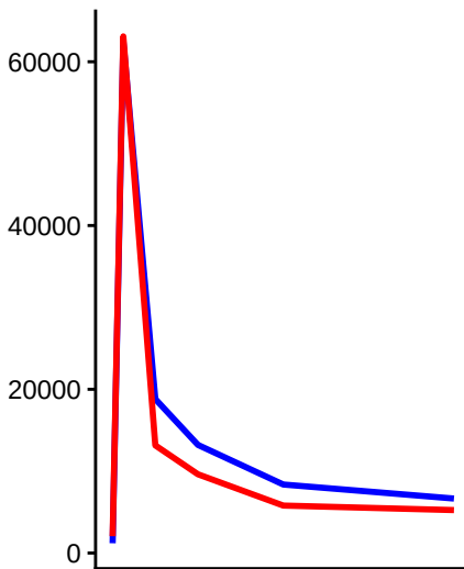
heat shock protein HSP 90-alpha LOC110235604
