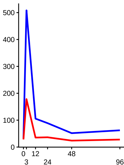
tumor necrosis factor receptor superfamily member 1A LOC110234017
