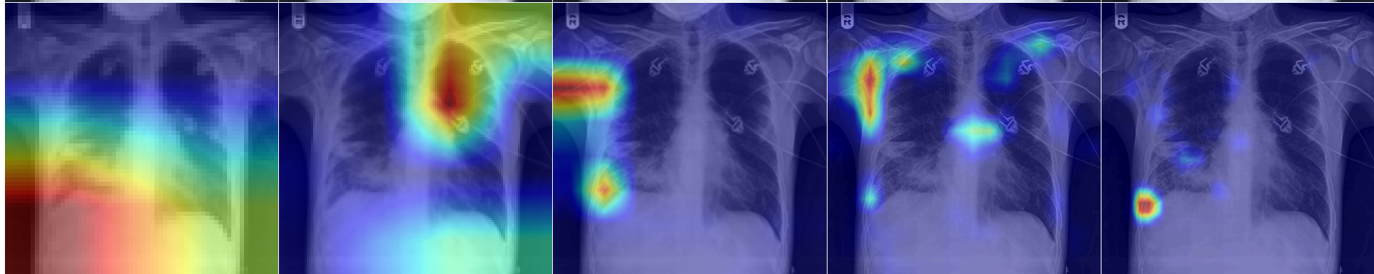
GradCAM
