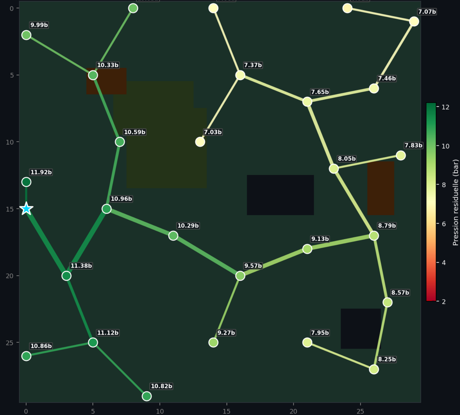
Pressions (Darcy-Weisbach + Colebrook-White)
