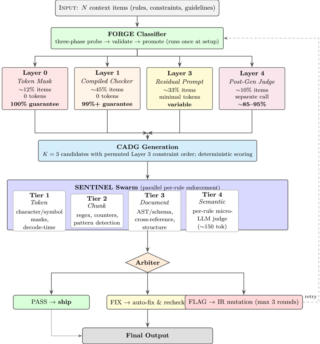
Figure 1: CPGA+SENTINEL combined architecture. N context items are classified by FORGE into four enforcement layers (CPGA Layers 0, 1, 3, 4 — Layer 2 reserved for activation steering, see Section 3.2). Only Layer 3 items ( \sim 33\% ) enter the LLM prompt; Layers 0, 1, and 4 enforce externally. CADG generates K = 3 candidates with permuted Layer 3 constraint order. The SENTINEL swarm runs four tiers (Token/Chunk/Document/Semantic) concurrently, corresponding to CPGA Layers 0/1/3/4 respectively. The Arbiter collects verdicts and routes failures to auto-fix (Tiers 1–3, fully deterministic) or IR-level mutation (max 3 rounds).
