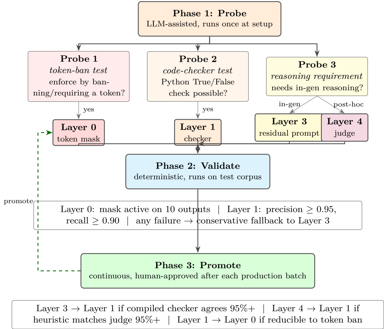
Figure 2: FORGE three-phase classification protocol. Phase 1 (Probe) runs three hierarchical LLM-assisted tests and assigns each context item to Layer 0, 1, 3, or 4; earlier (cheaper) probes win ties. Phase 2 (Validate) runs deterministic checks on a test corpus and demotes any item that fails its assigned layer to Layer 3 (conservative fallback, Principle 1). Phase 3 (Promote) runs continuously after each production batch and moves items to cheaper layers when their checker/heuristic agrees with the more expensive oracle \geq 95\% of the time; all promotions require human approval.
