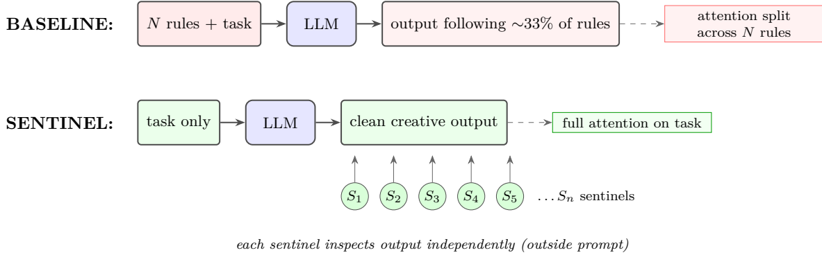
Figure 3: BASELINE vs. SENTINEL enforcement topology. In the baseline, all N enforcement rules share the LLM prompt, so attention is split across creative task and rule-following. SENTINEL strips all enforcement from the prompt: the LLM sees only the task, while n independent sentinel agents inspect the output externally (tier-appropriate per rule). This eliminates enforcement-related context degradation (failure modes F1–F7, Section 2) by construction; the LLM’s attention budget is free for creative/reasoning work.
