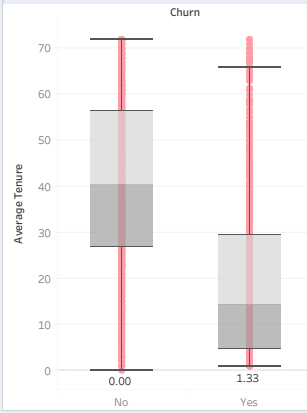
Churn by Tenure Bands
