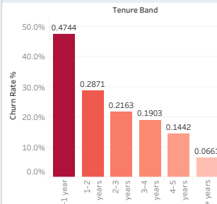
Churn by Tenure Bands
