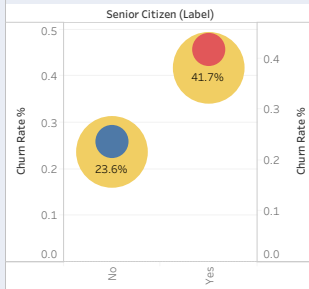
Senior Citizen Churn (Donut)
