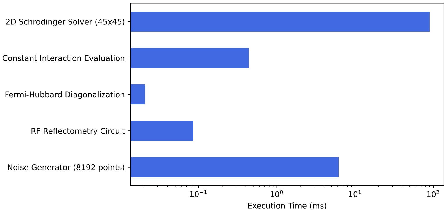
QuantumTwin Execution Time Benchmarks
