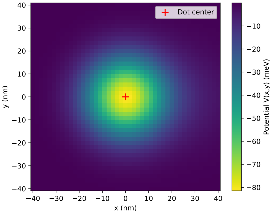
Electrostatic Potential Well
