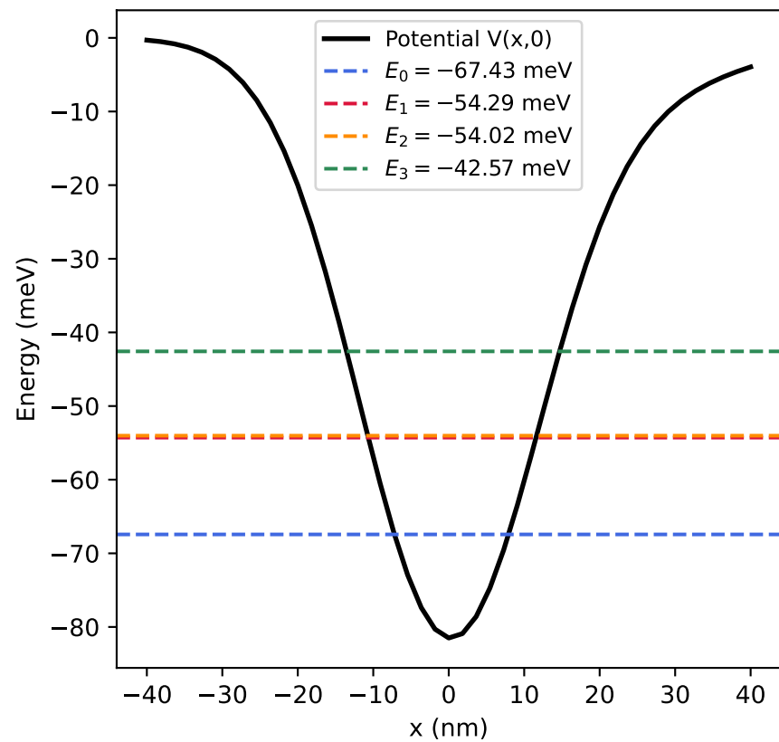
Cross-Section &amp; Bound States
