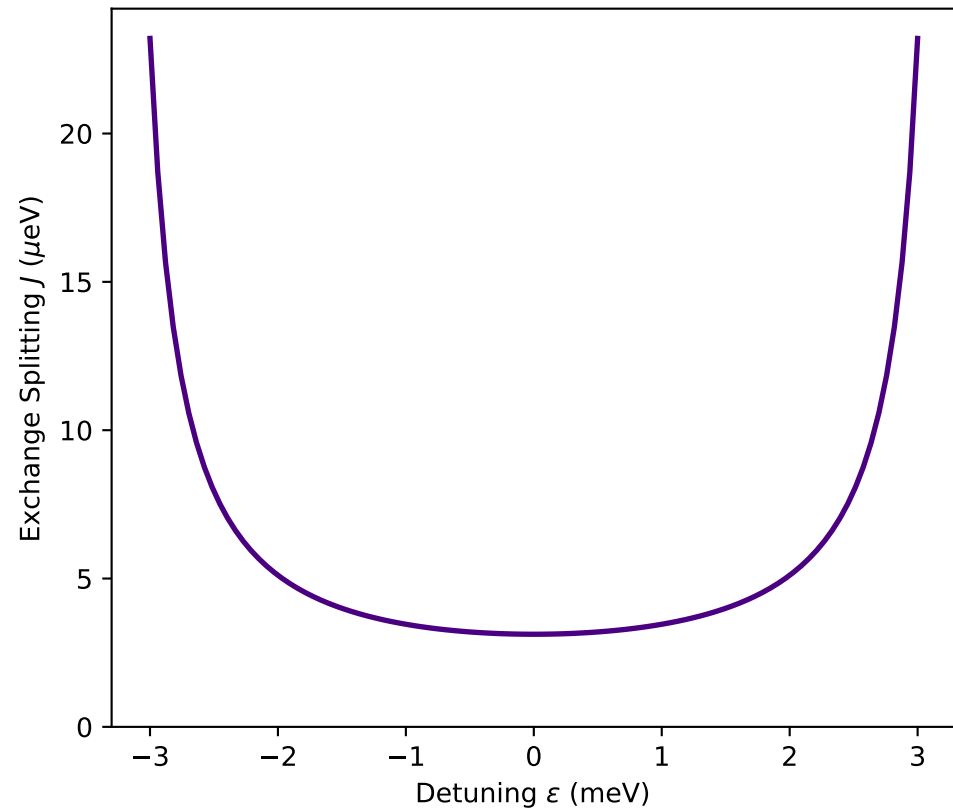
Singlet-Triplet Exchange J(\varepsilon)
