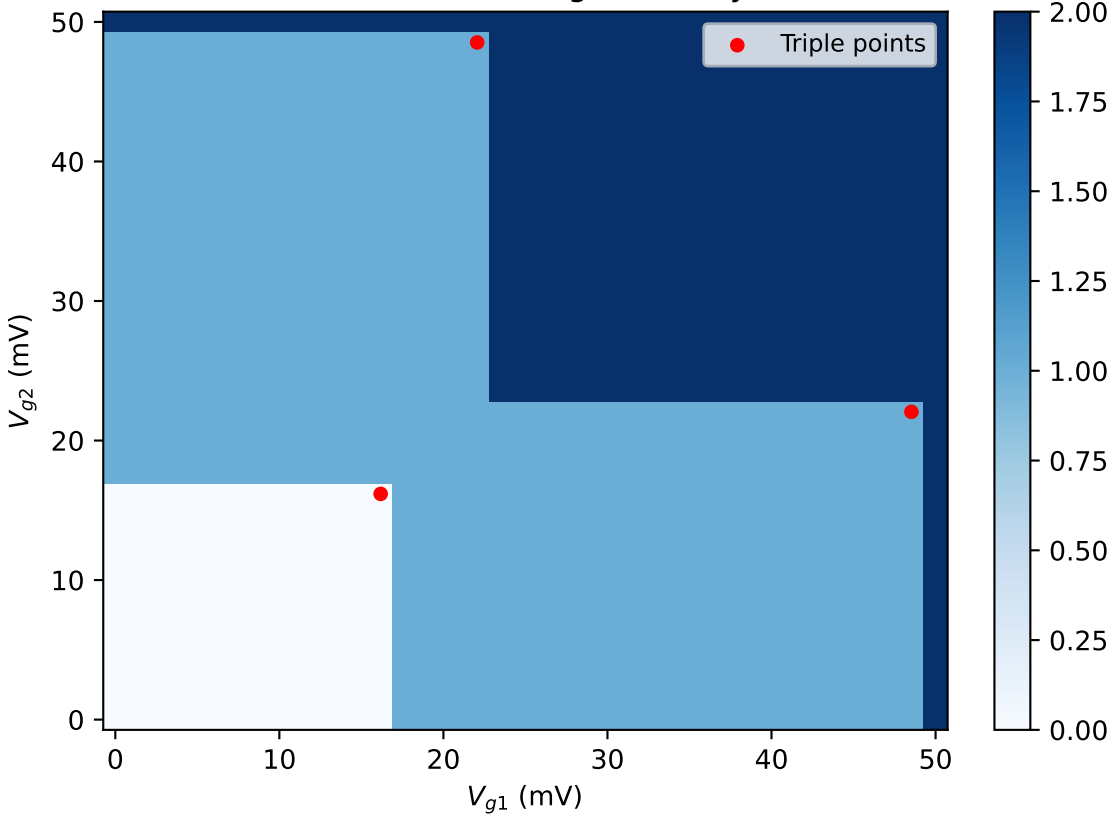
Double Dot Charge Stability
