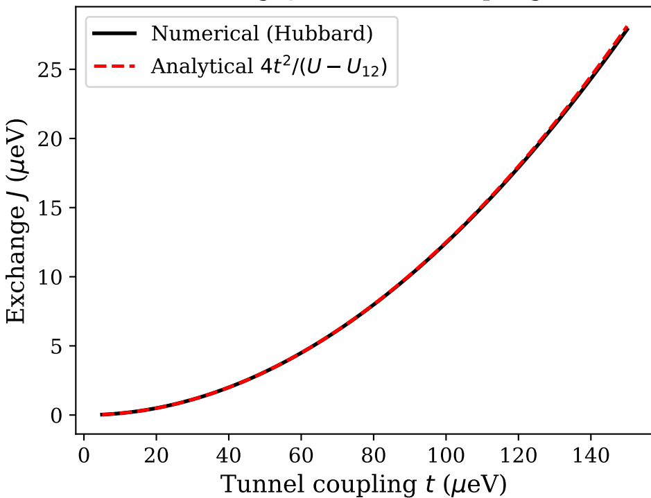
Exchange J vs Tunnel Coupling t
