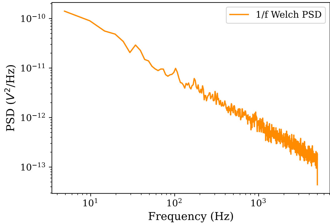
1/f Power Spectrum ( \alpha_{fit} = 0.976 , R^2 = 0.896 )
