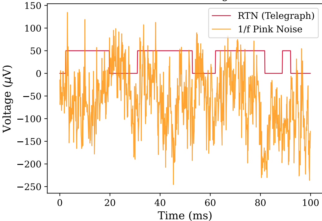
Time-Domain Noise Signatures
